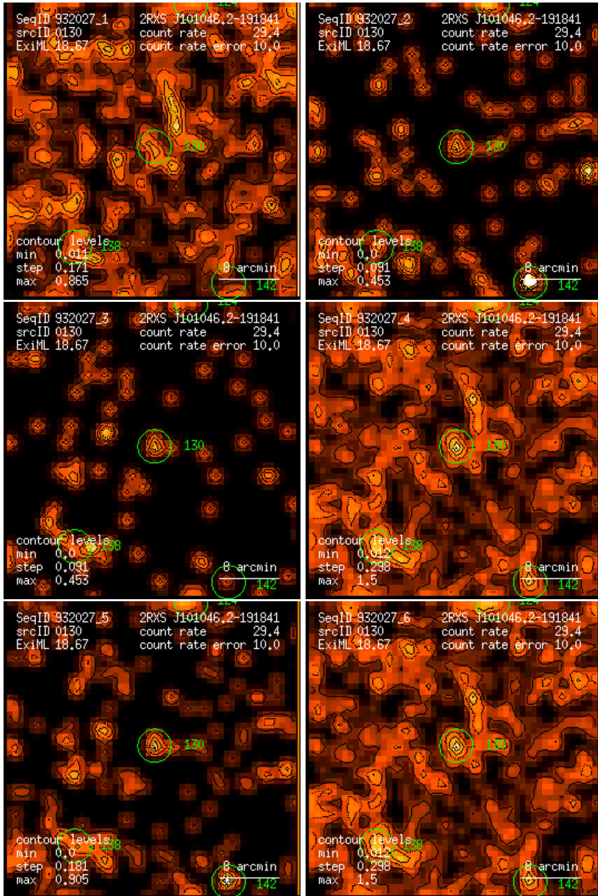
Figure 130: RASS 932027: detection 0130: band rate images, Gaussian filter: (1) PSPC channels 11 – 41, (2) 52 – 90, (3) 91 – 201, (4) 11 – 235, (5) 52 – 201, (6) 11 – 201. Broad band rates in counts/ks. Band rate contour levels in counts/ks/arcmin 2 .
