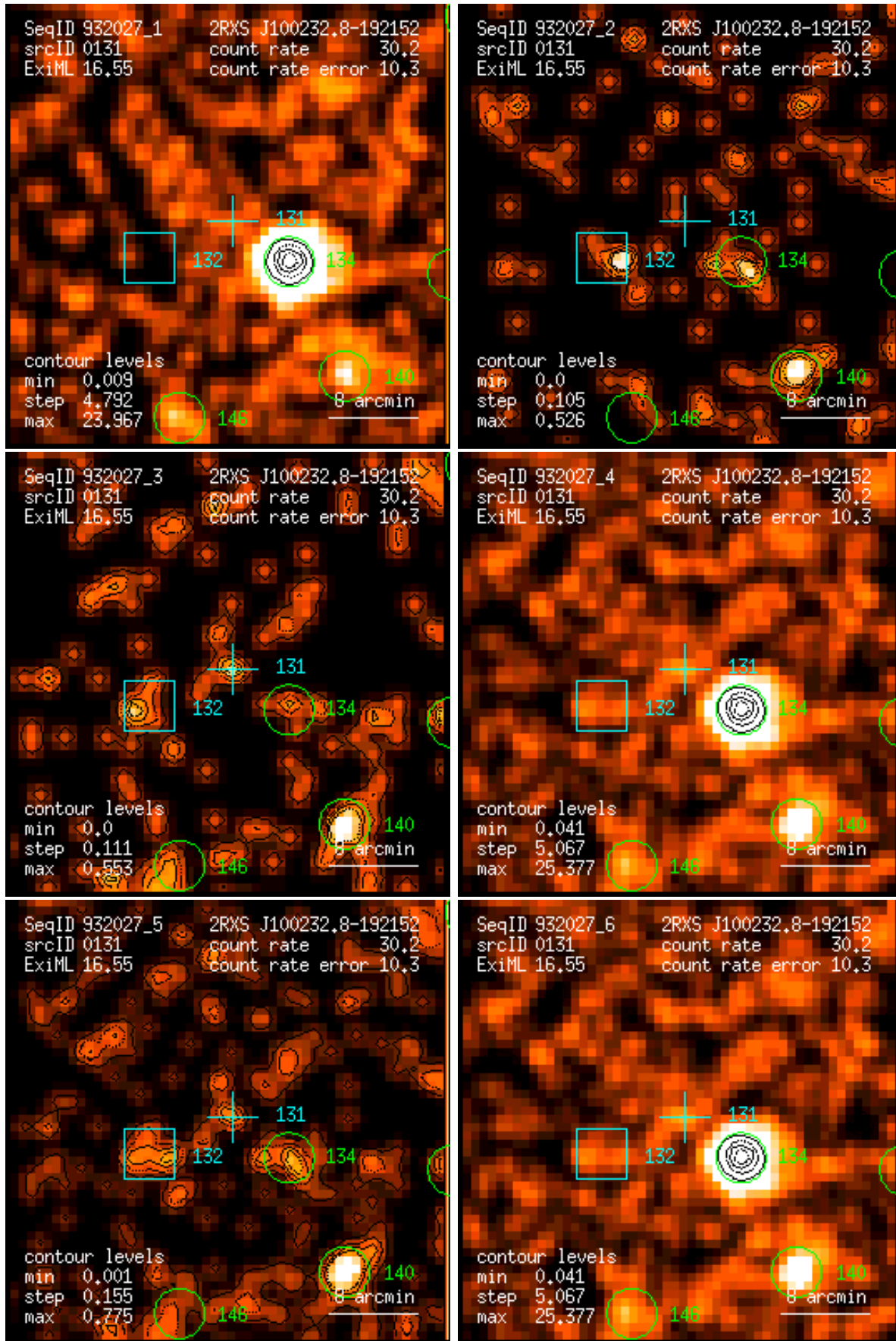
Figure 131: RASS 932027: detection 0131: band rate images, Gaussian filter: (1) PSPC channels 11 – 41, (2) 52 – 90, (3) 91 – 201, (4) 11 – 235, (5) 52 – 201, (6) 11 – 201. Broad band rates in counts/ks. Band rate contour levels in counts/ks/arcmin 2 .
