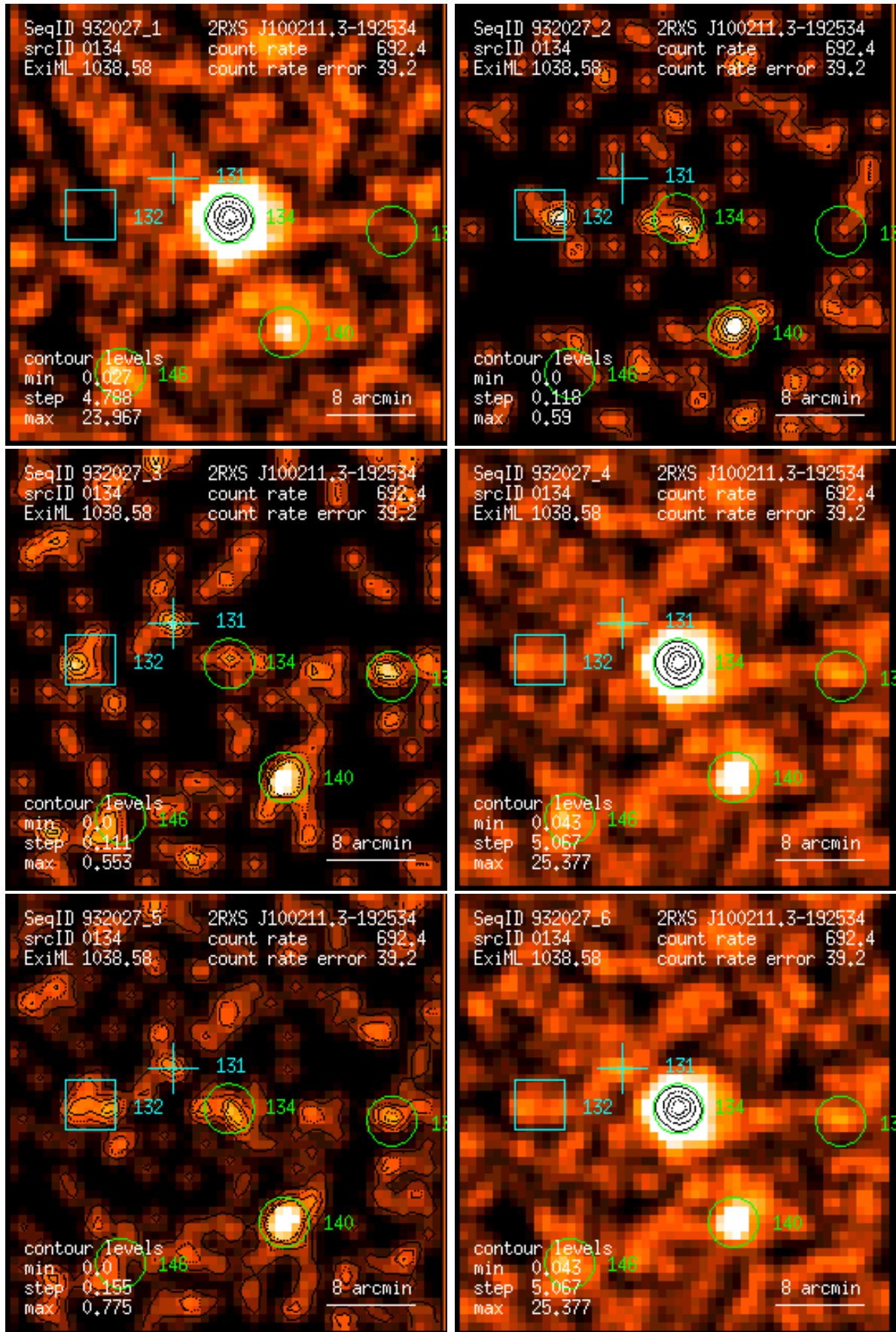
Figure 134: RASS 932027: detection 0134: band rate images, Gaussian filter: (1) PSPC channels 11 – 41, (2) 52 – 90, (3) 91 – 201, (4) 11 – 235, (5) 52 – 201, (6) 11 – 201. Broad band rates in counts/ks. Band rate contour levels in counts/ks/arcmin 2 .
