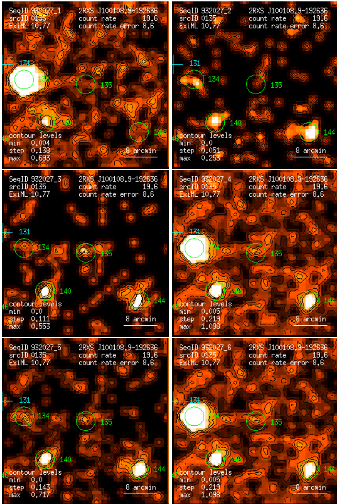
Figure 135: RASS 932027: detection 0135: band rate images, Gaussian filter: (1) PSPC channels 11 – 41, (2) 52 – 90, (3) 91 – 201, (4) 11 – 235, (5) 52 – 201, (6) 11 – 201. Broad band rates in counts/ks. Band rate contour levels in counts/ks/arcmin 2 .
