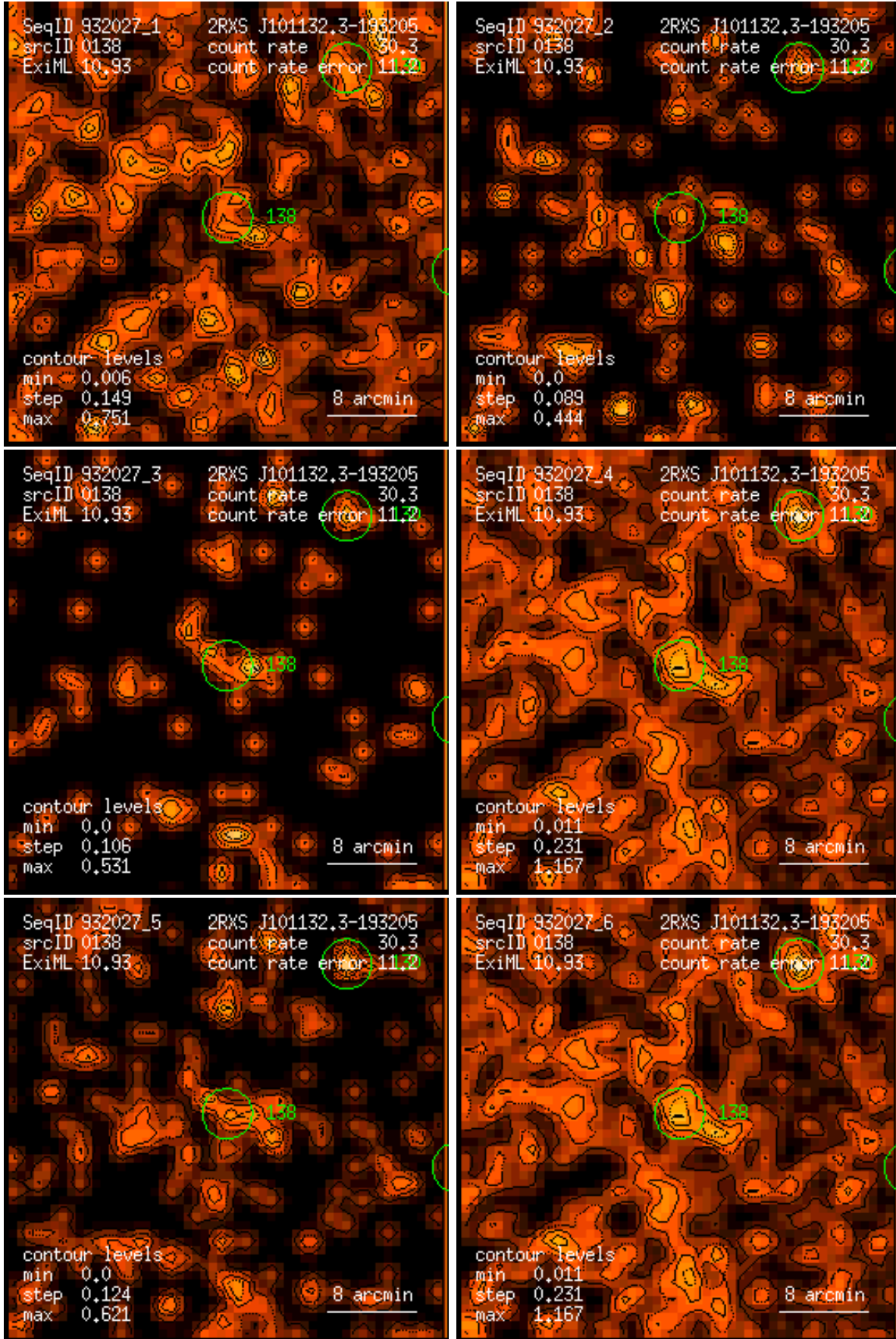
Figure 138: RASS 932027: detection 0138: band rate images, Gaussian filter: (1) PSPC channels 11 – 41, (2) 52 – 90, (3) 91 – 201, (4) 11 – 235, (5) 52 – 201, (6) 11 – 201. Broad band rates in counts/ks. Band rate contour levels in counts/ks/arcmin 2 .
