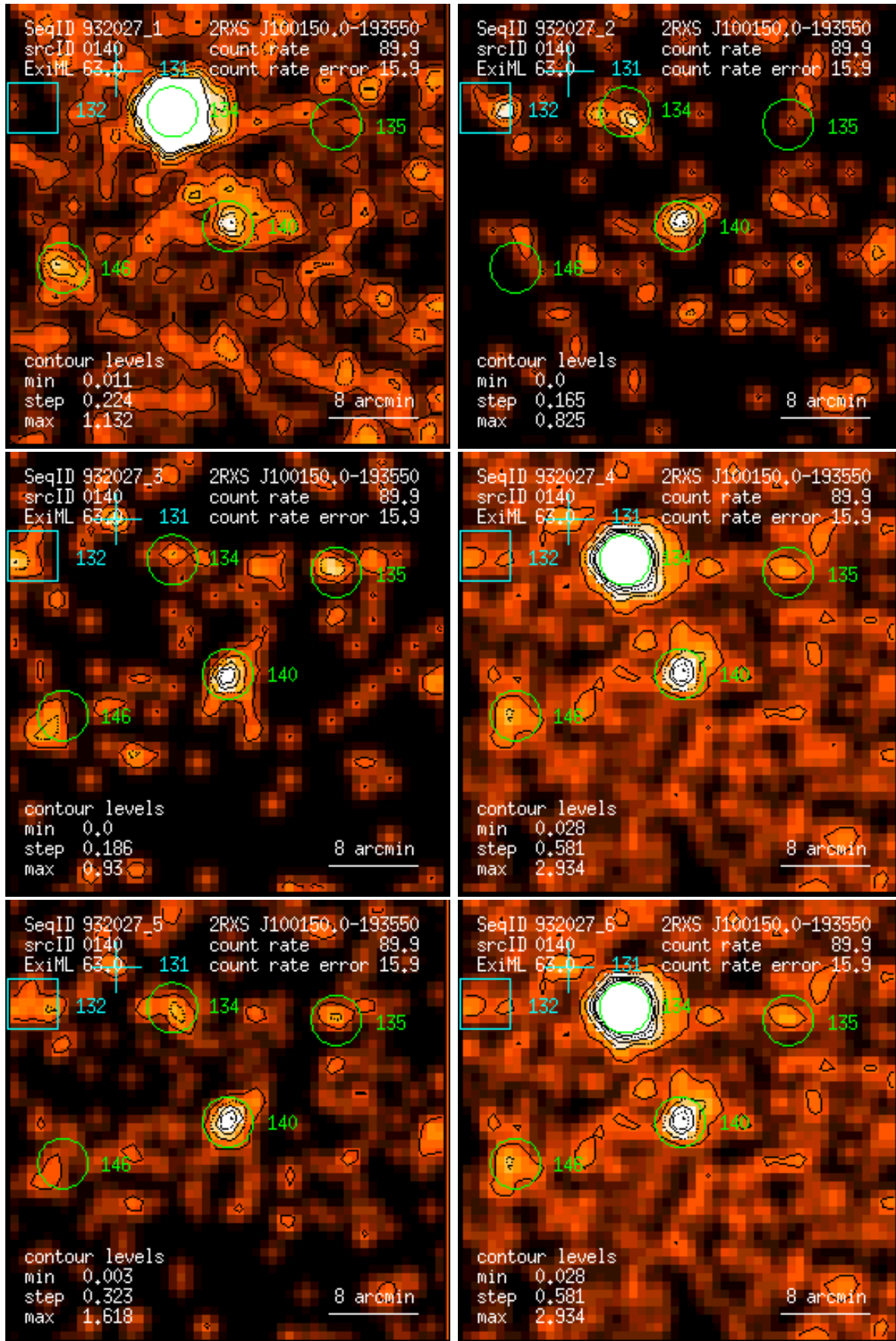
Figure 140: RASS 932027: detection 0140: band rate images, Gaussian filter: (1) PSPC channels 11 – 41, (2) 52 – 90, (3) 91 – 201, (4) 11 – 235, (5) 52 – 201, (6) 11 – 201. Broad band rates in counts/ks. Band rate contour levels in counts/ks/arcmin 2 .
