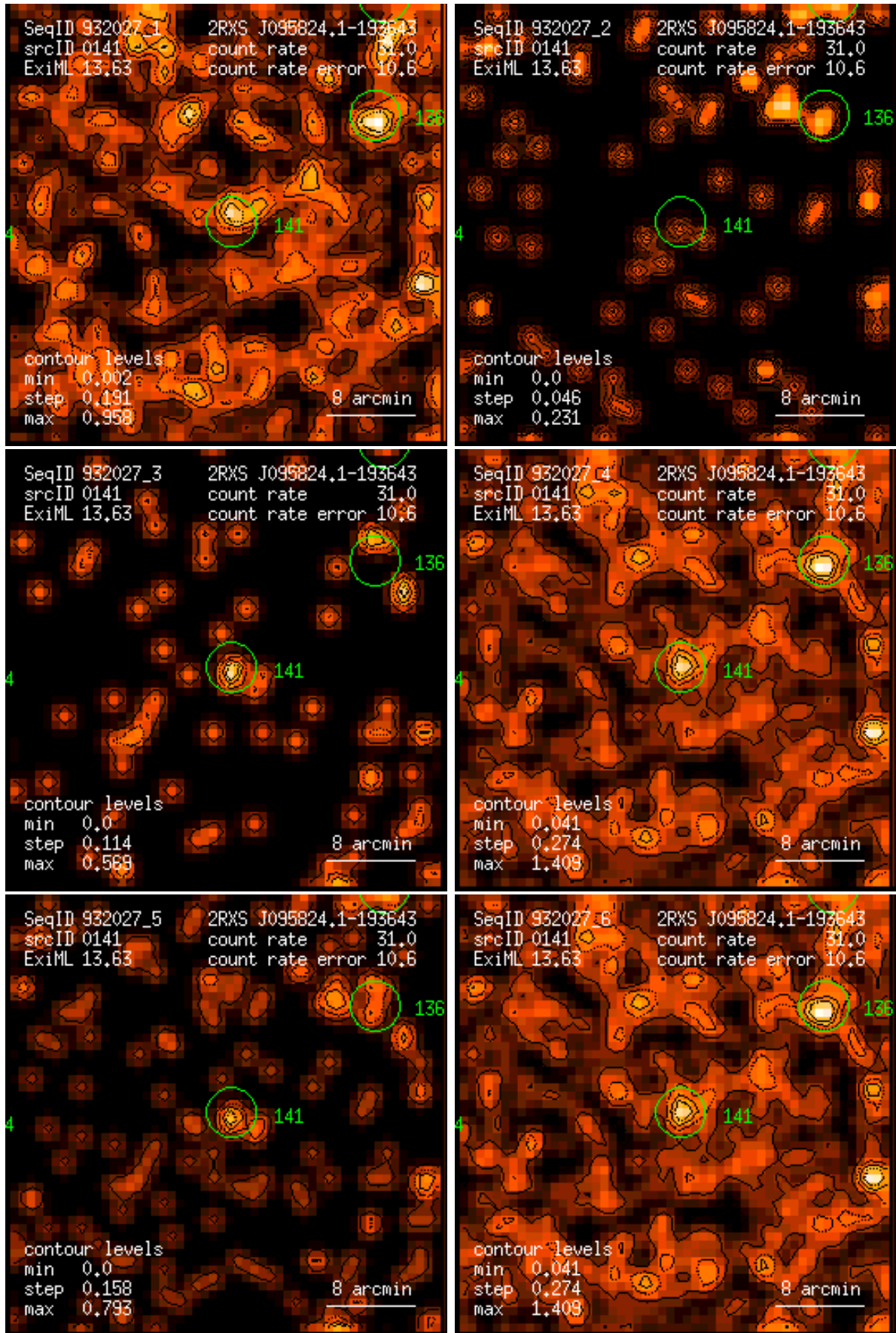
Figure 141: RASS 932027: detection 0141: band rate images, Gaussian filter: (1) PSPC channels 11 – 41, (2) 52 – 90, (3) 91 – 201, (4) 11 – 235, (5) 52 – 201, (6) 11 – 201. Broad band rates in counts/ks. Band rate contour levels in counts/ks/arcmin 2 .
