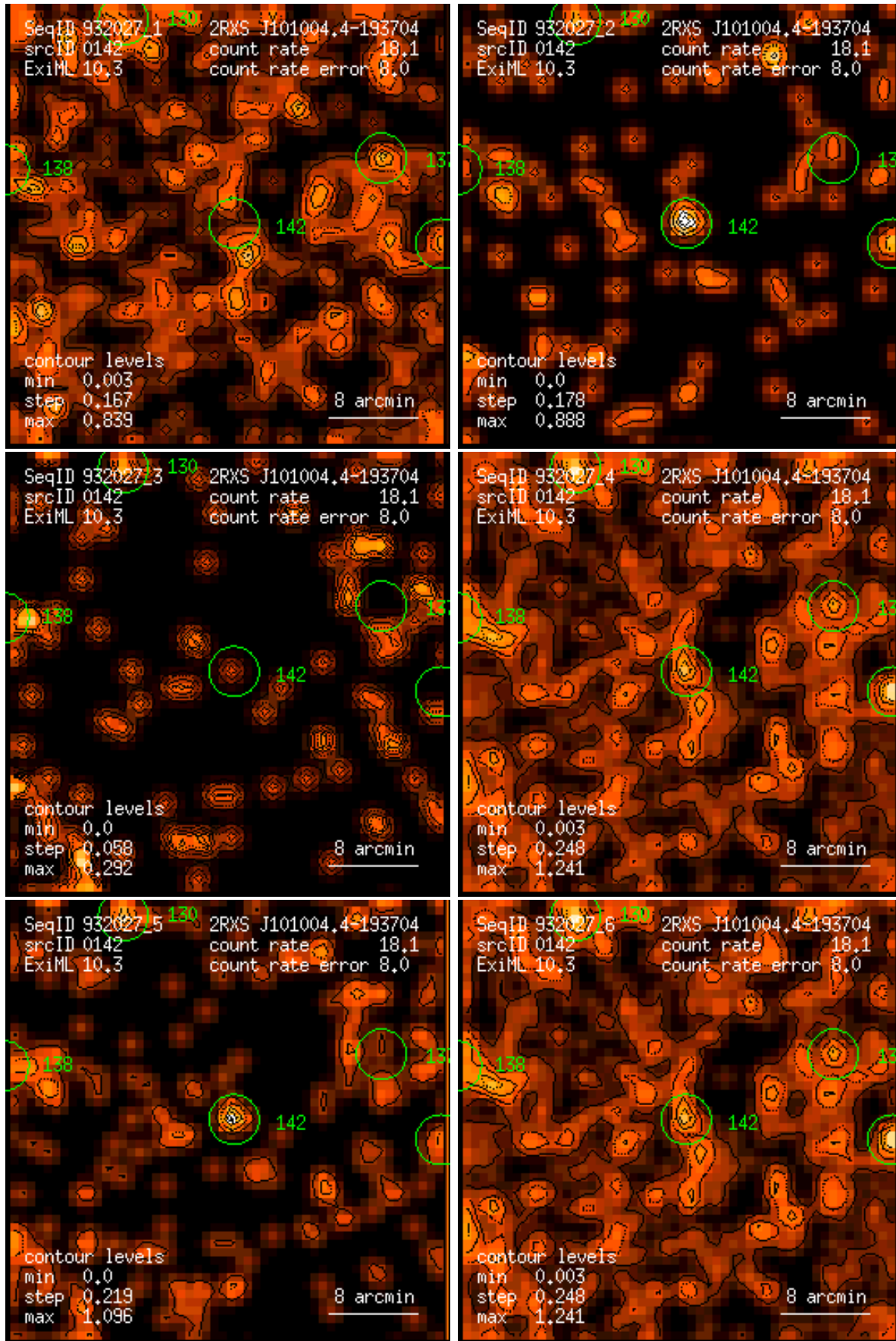
Figure 142: RASS 932027: detection 0142: band rate images, Gaussian filter: (1) PSPC channels 11 – 41, (2) 52 – 90, (3) 91 – 201, (4) 11 – 235, (5) 52 – 201, (6) 11 – 201. Broad band rates in counts/ks. Band rate contour levels in counts/ks/arcmin 2 .
