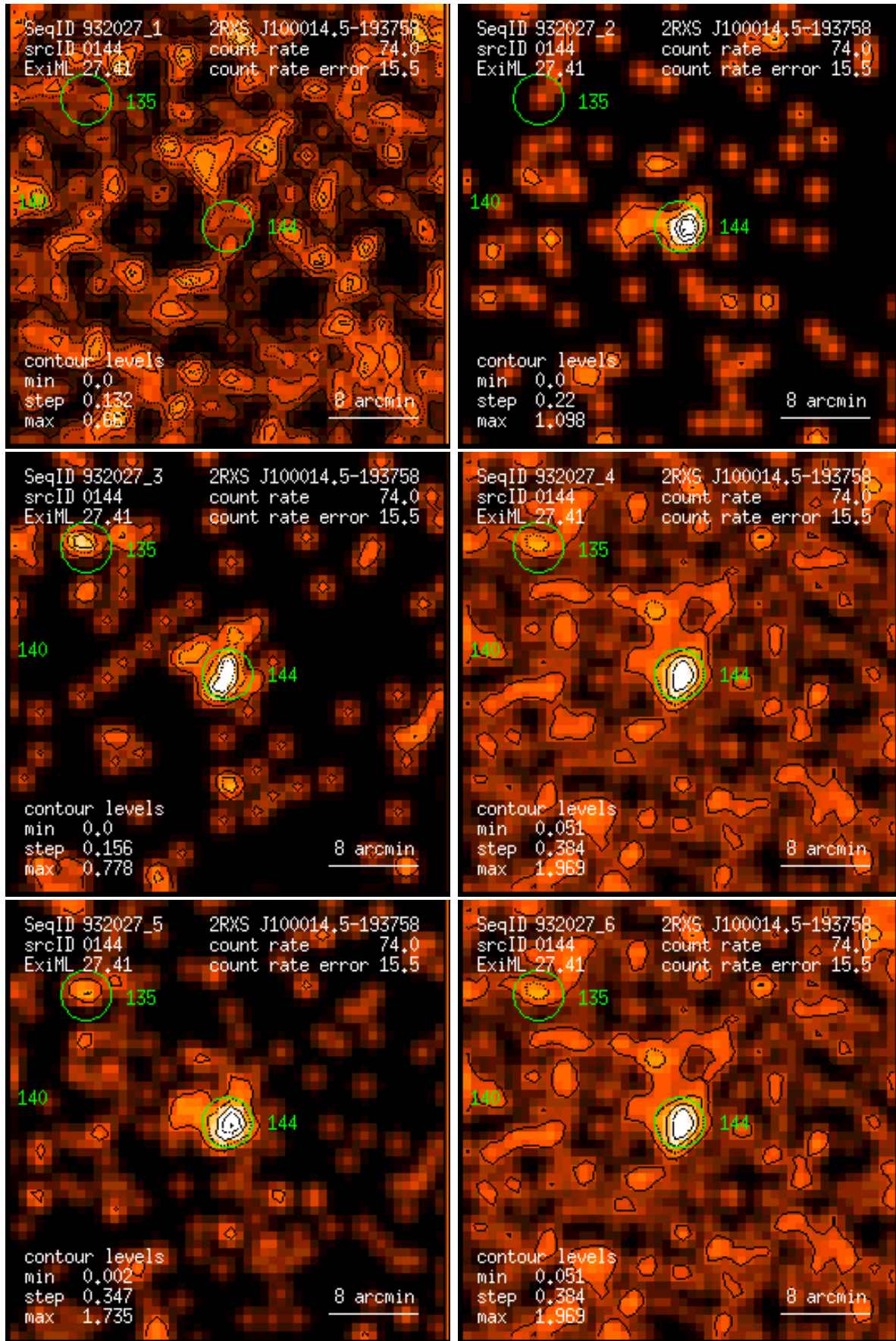
Figure 144: RASS 932027: detection 0144: band rate images, Gaussian filter: (1) PSPC channels 11 – 41, (2) 52 – 90, (3) 91 – 201, (4) 11 – 235, (5) 52 – 201, (6) 11 – 201. Broad band rates in counts/ks. Band rate contour levels in counts/ks/arcmin 2 .
