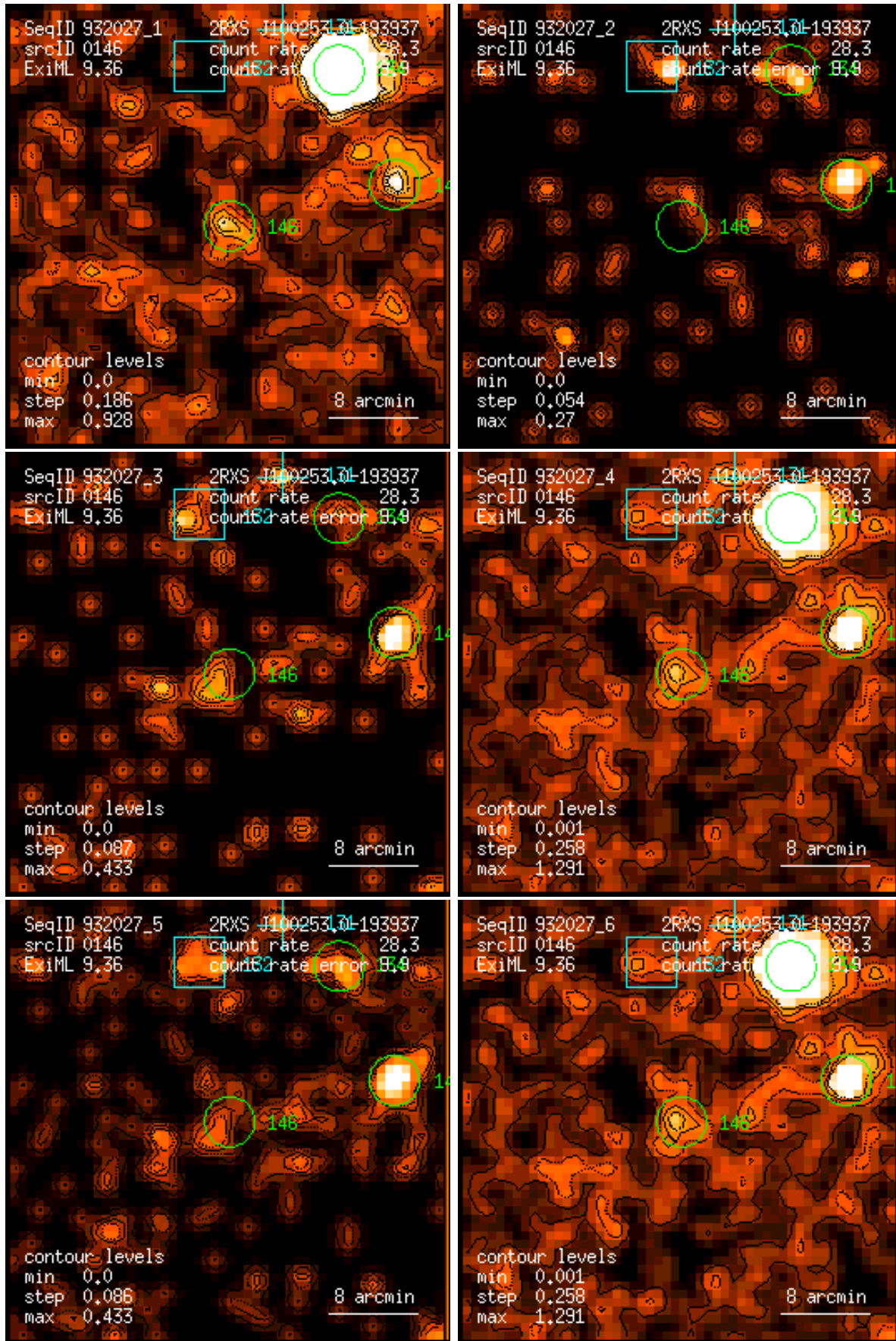
Figure 146: RASS 932027: detection 0146: band rate images, Gaussian filter: (1) PSPC channels 11 – 41, (2) 52 – 90, (3) 91 – 201, (4) 11 – 235, (5) 52 – 201, (6) 11 – 201. Broad band rates in counts/ks. Band rate contour levels in counts/ks/arcmin 2 .
