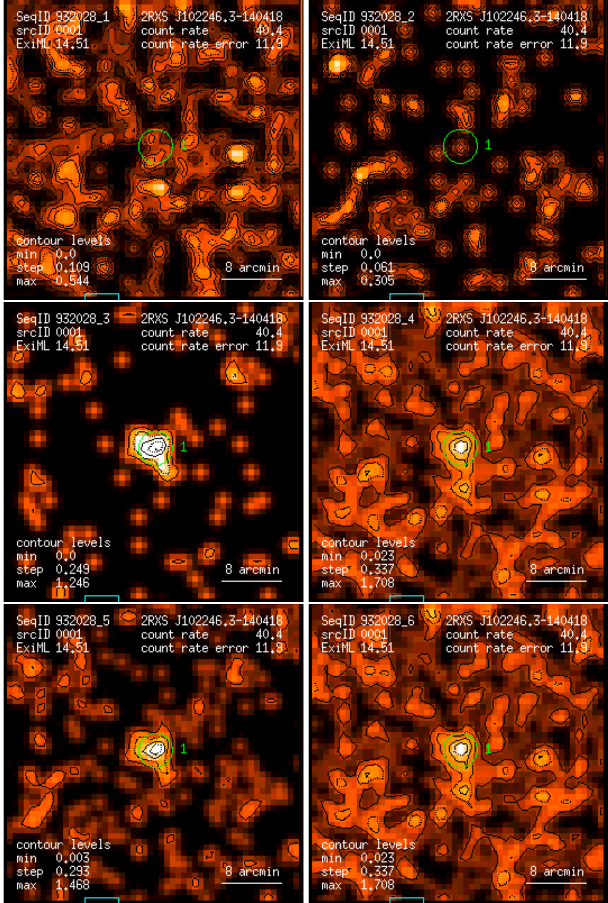
Figure 1: RASS 932028: detection 0001: band rate images, Gaussian filter: (1) PSPC channels 11 – 41, (2) 52 – 90, (3) 91 – 201, (4) 11 – 235, (5) 52 – 201, (6) 11 – 201. Broad band rates in counts/ks. Band rate contour levels in counts/ks/arcmin 2 .
