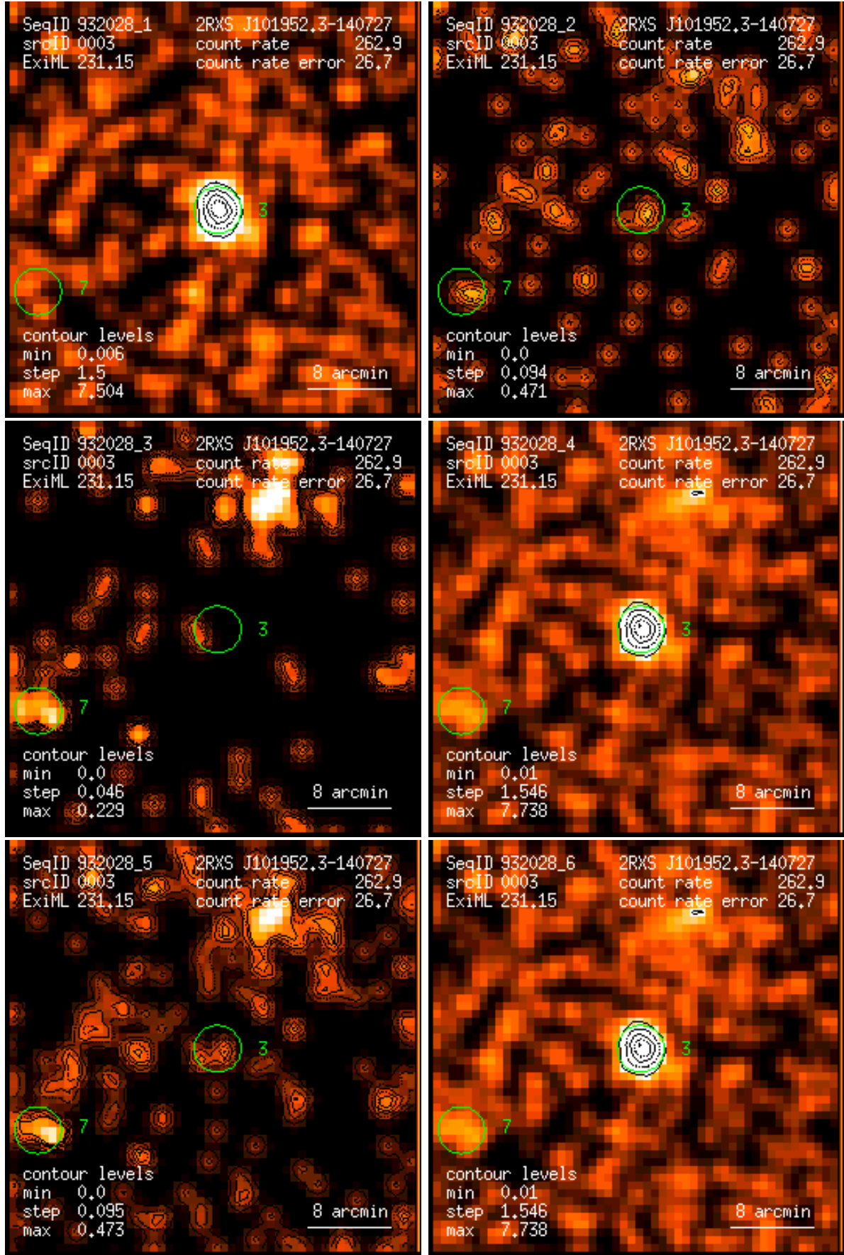
Figure 3: RASS 932028: detection 0003: band rate images, Gaussian filter: (1) PSPC channels 11 – 41, (2) 52 – 90, (3) 91 – 201, (4) 11 – 235, (5) 52 – 201, (6) 11 – 201. Broad band rates in counts/ks. Band rate contour levels in counts/ks/arcmin 2 .
