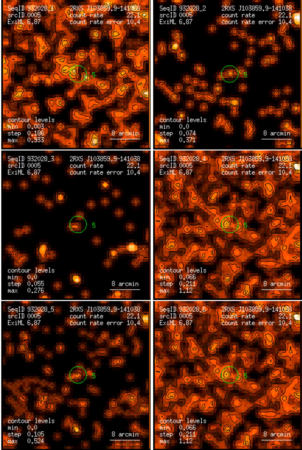
Figure 5: RASS 932028: detection 0005: band rate images, Gaussian filter: (1) PSPC channels 11 – 41, (2) 52 – 90, (3) 91 – 201, (4) 11 – 235, (5) 52 – 201, (6) 11 – 201. Broad band rates in counts/ks. Band rate contour levels in counts/ks/arcmin 2 .
