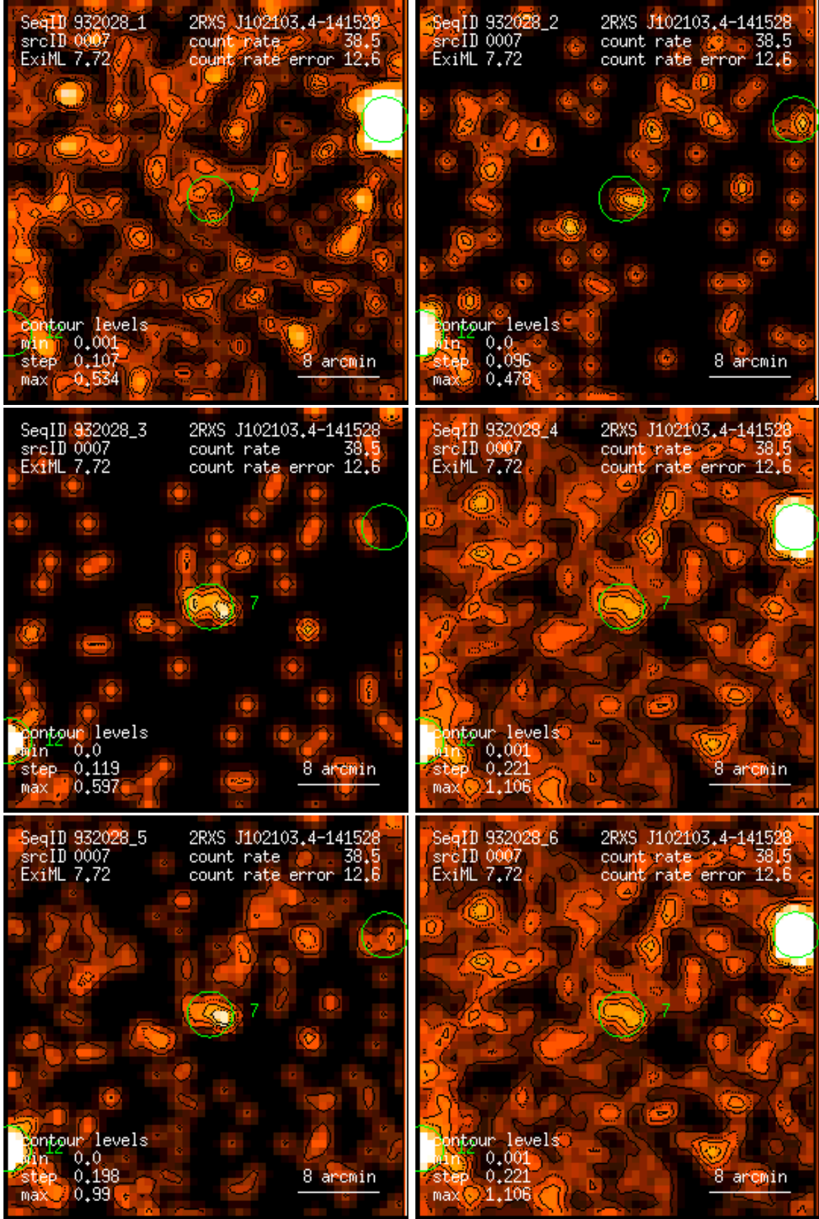
Figure 7: RASS 932028: detection 0007: band rate images, Gaussian filter: (1) PSPC channels 11 – 41, (2) 52 – 90, (3) 91 – 201, (4) 11 – 235, (5) 52 – 201, (6) 11 – 201. Broad band rates in counts/ks. Band rate contour levels in counts/ks/arcmin 2 .
