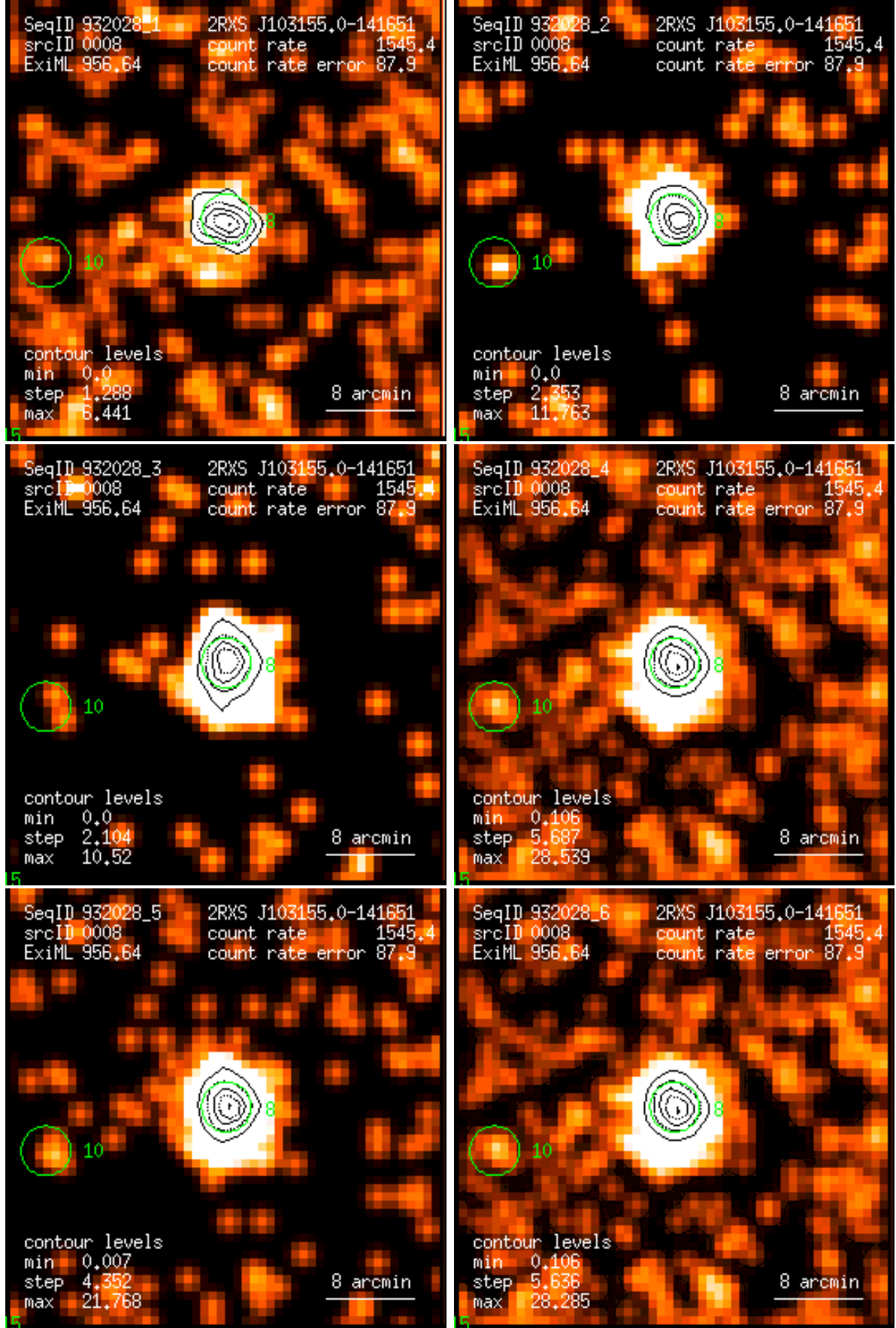
Figure 8: RASS 932028: detection 0008: band rate images, Gaussian filter: (1) PSPC channels 11 – 41, (2) 52 – 90, (3) 91 – 201, (4) 11 – 235, (5) 52 – 201, (6) 11 – 201. Broad band rates in counts/ks. Band rate contour levels in counts/ks/arcmin 2 .
