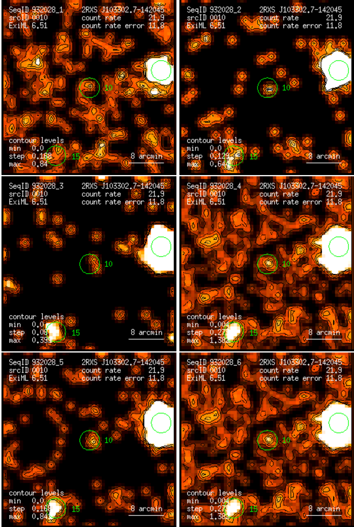
Figure 10: RASS 932028: detection 0010: band rate images, Gaussian filter: (1) PSPC channels 11 – 41, (2) 52 – 90, (3) 91 – 201, (4) 11 – 235, (5) 52 – 201, (6) 11 – 201. Broad band rates in counts/ks. Band rate contour levels in counts/ks/arcmin 2 .
