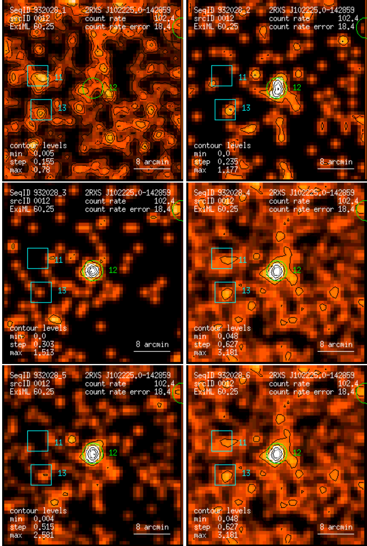
Figure 12: RASS 932028: detection 0012: band rate images, Gaussian filter: (1) PSPC channels 11 – 41, (2) 52 – 90, (3) 91 – 201, (4) 11 – 235, (5) 52 – 201, (6) 11 – 201. Broad band rates in counts/ks. Band rate contour levels in counts/ks/arcmin 2 .
