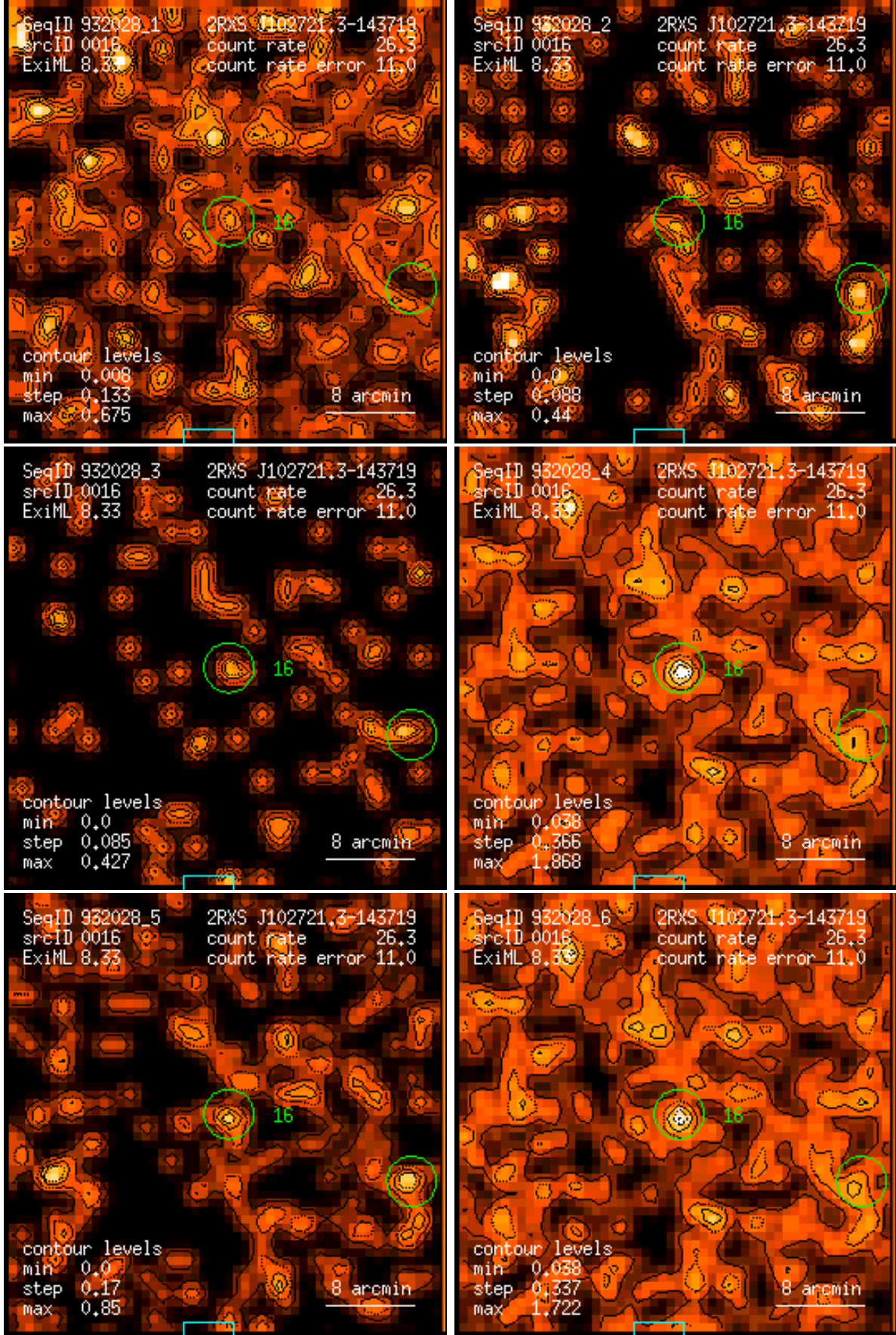
Figure 16: RASS 932028: detection 0016: band rate images, Gaussian filter: (1) PSPC channels 11 – 41, (2) 52 – 90, (3) 91 – 201, (4) 11 – 235, (5) 52 – 201, (6) 11 – 201. Broad band rates in counts/ks. Band rate contour levels in counts/ks/arcmin 2 .
