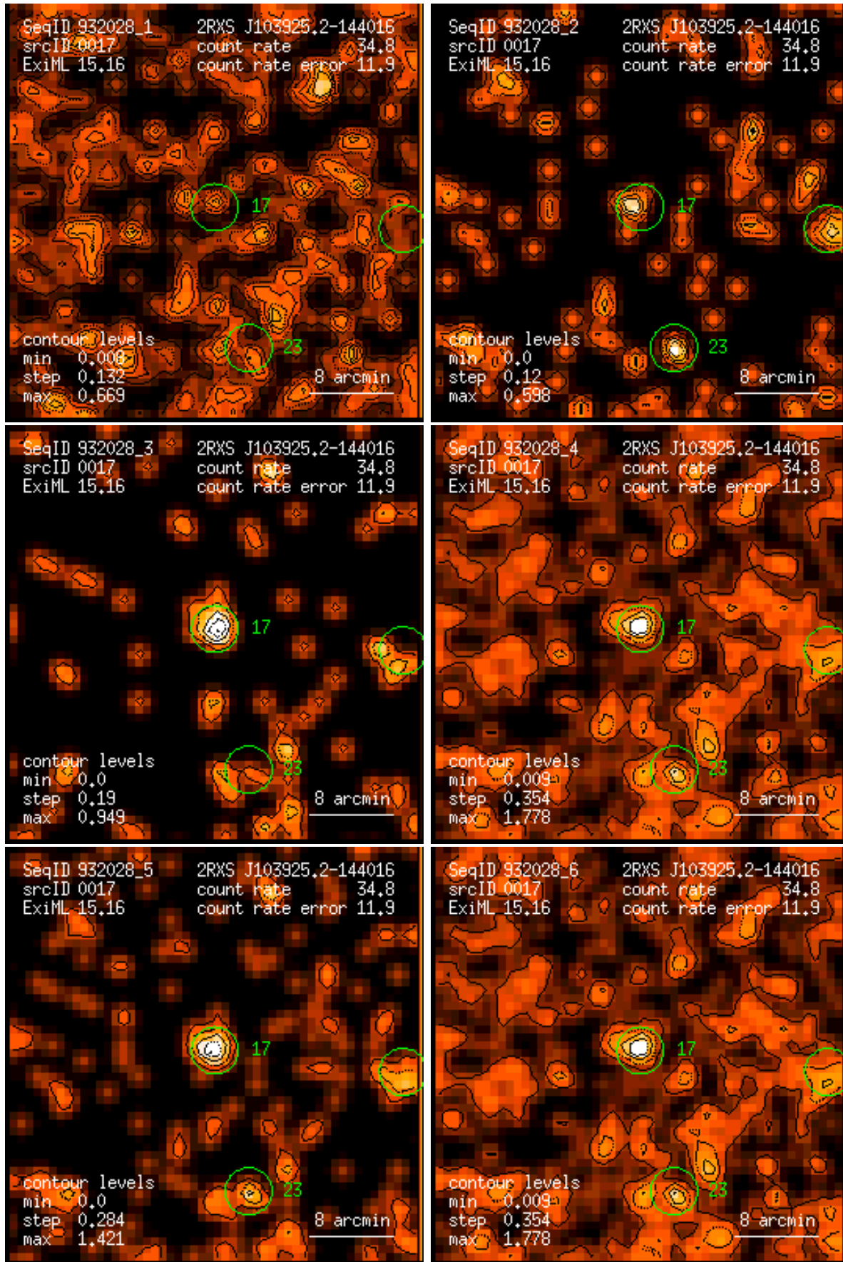
Figure 17: RASS 932028: detection 0017: band rate images, Gaussian filter: (1) PSPC channels 11 – 41, (2) 52 – 90, (3) 91 – 201, (4) 11 – 235, (5) 52 – 201, (6) 11 – 201. Broad band rates in counts/ks. Band rate contour levels in counts/ks/arcmin 2 .
