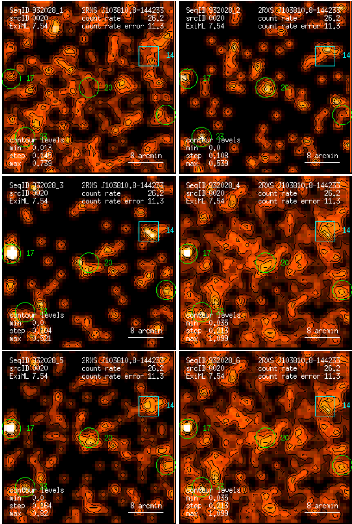
Figure 20: RASS 932028: detection 0020: band rate images, Gaussian filter: (1) PSPC channels 11 – 41, (2) 52 – 90, (3) 91 – 201, (4) 11 – 235, (5) 52 – 201, (6) 11 – 201. Broad band rates in counts/ks. Band rate contour levels in counts/ks/arcmin 2 .
