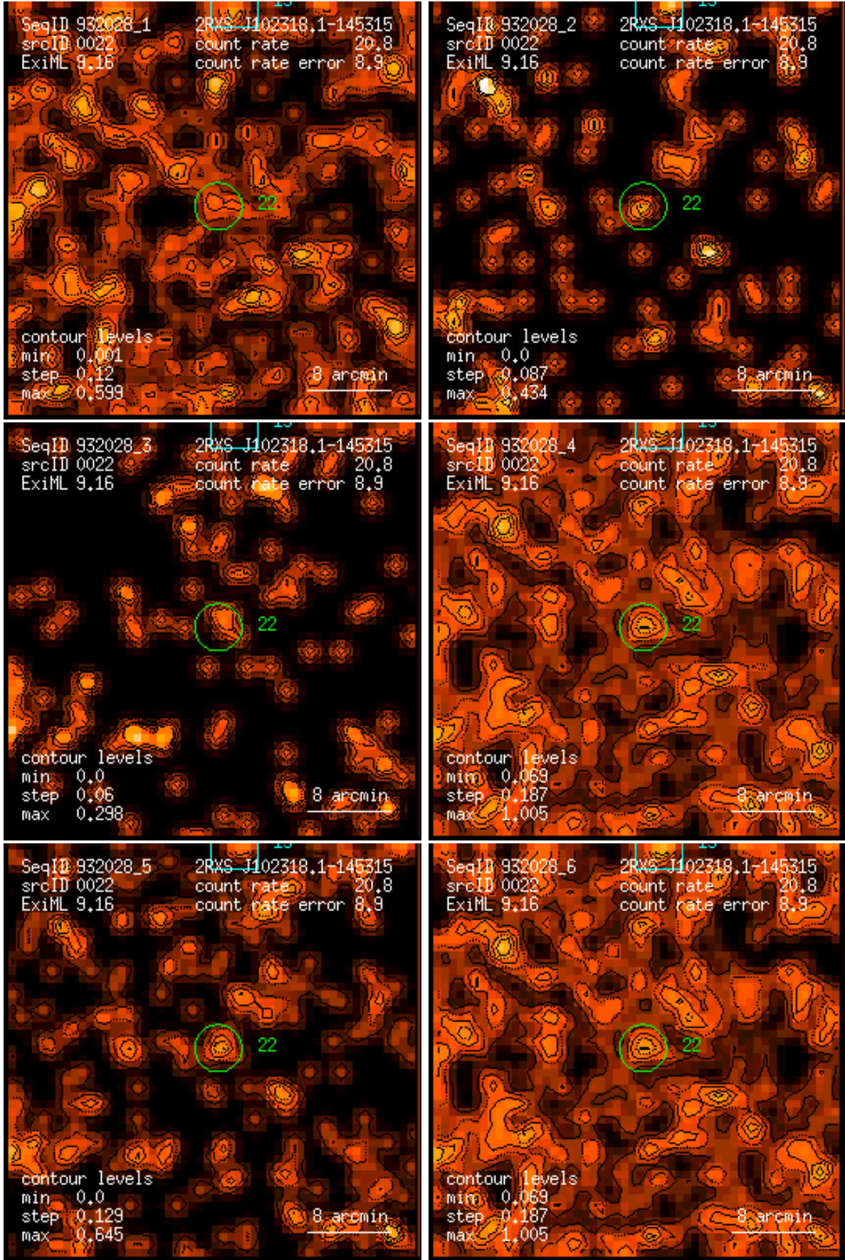
Figure 22: RASS 932028: detection 0022: band rate images, Gaussian filter: (1) PSPC channels 11 – 41, (2) 52 – 90, (3) 91 – 201, (4) 11 – 235, (5) 52 – 201, (6) 11 – 201. Broad band rates in counts/ks. Band rate contour levels in counts/ks/arcmin 2 .
