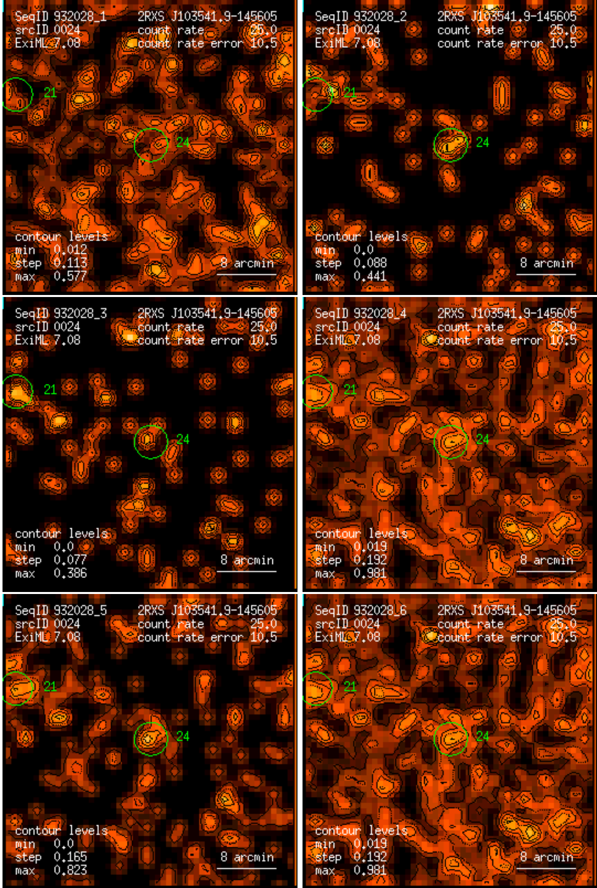
Figure 24: RASS 932028: detection 0024: band rate images, Gaussian filter: (1) PSPC channels 11 – 41, (2) 52 – 90, (3) 91 – 201, (4) 11 – 235, (5) 52 – 201, (6) 11 – 201. Broad band rates in counts/ks. Band rate contour levels in counts/ks/arcmin 2 .
