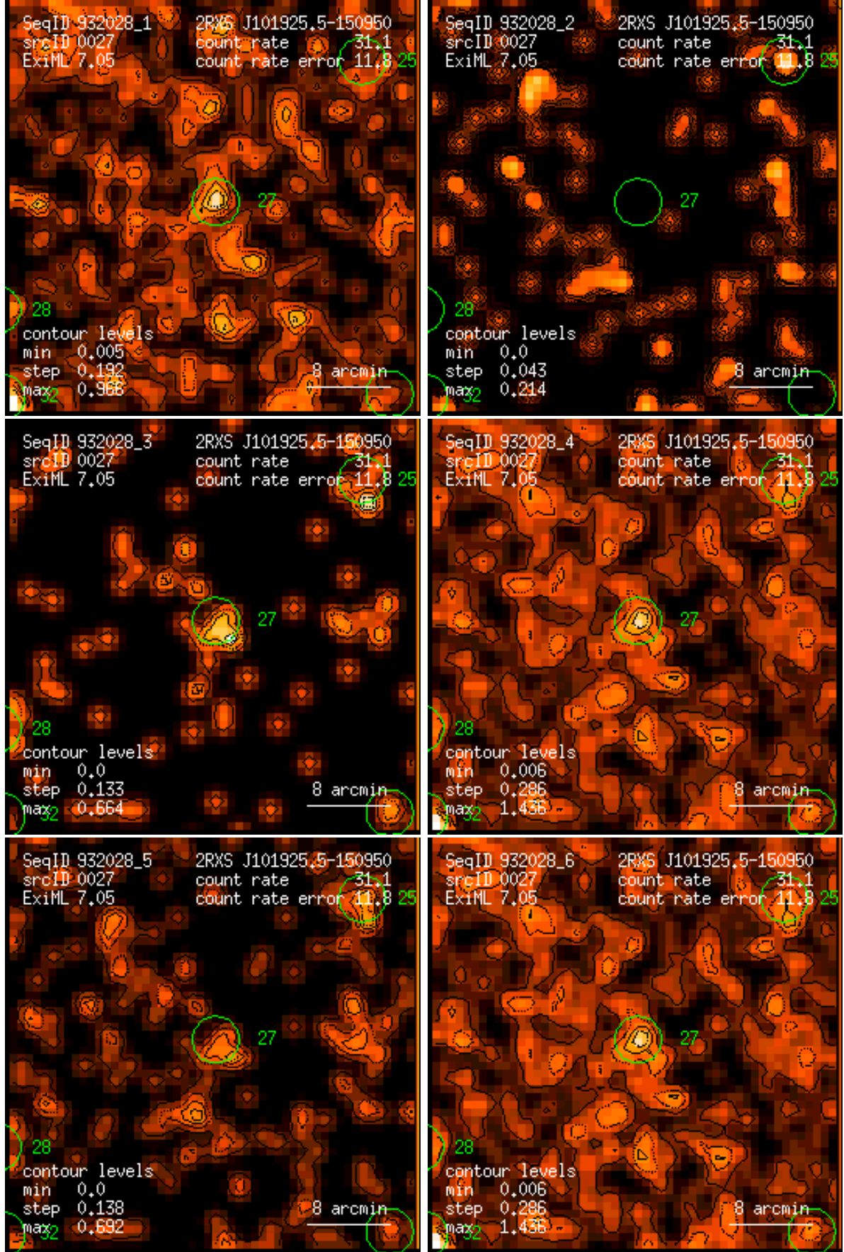
Figure 27: RASS 932028: detection 0027: band rate images, Gaussian filter: (1) PSPC channels 11 – 41, (2) 52 – 90, (3) 91 – 201, (4) 11 – 235, (5) 52 – 201, (6) 11 – 201. Broad band rates in counts/ks. Band rate contour levels in counts/ks/arcmin 2 .
