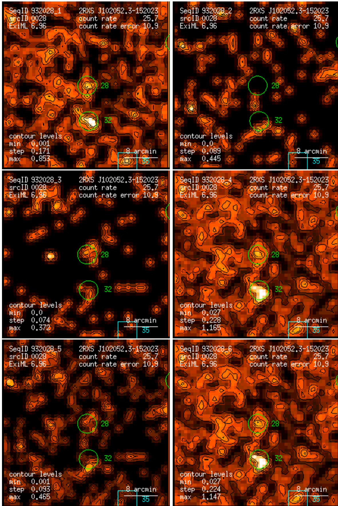
Figure 28: RASS 932028: detection 0028: band rate images, Gaussian filter: (1) PSPC channels 11 – 41, (2) 52 – 90, (3) 91 – 201, (4) 11 – 235, (5) 52 – 201, (6) 11 – 201. Broad band rates in counts/ks. Band rate contour levels in counts/ks/arcmin 2 .
