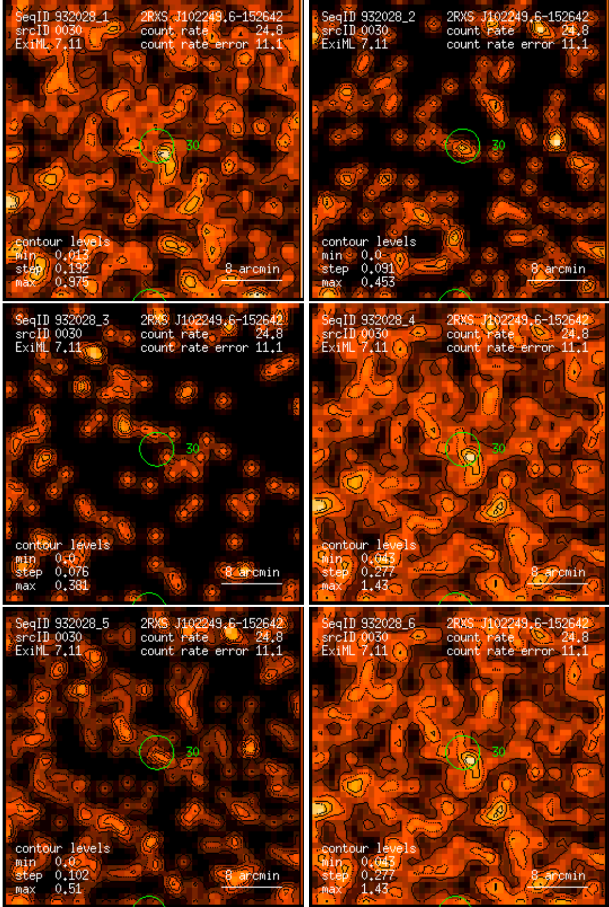
Figure 30: RASS 932028: detection 0030: band rate images, Gaussian filter: (1) PSPC channels 11 – 41, (2) 52 – 90, (3) 91 – 201, (4) 11 – 235, (5) 52 – 201, (6) 11 – 201. Broad band rates in counts/ks. Band rate contour levels in counts/ks/arcmin 2 .
