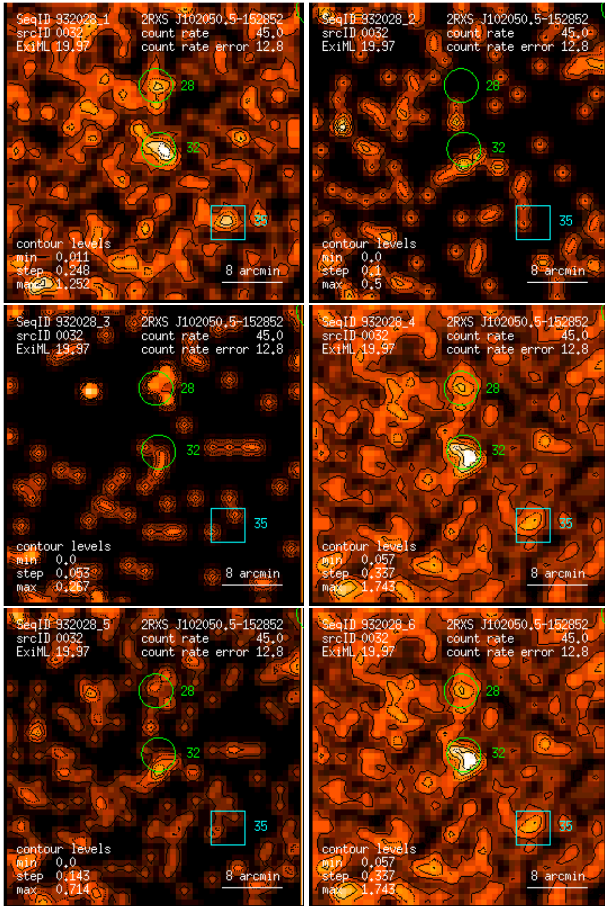
Figure 32: RASS 932028: detection 0032: band rate images, Gaussian filter: (1) PSPC channels 11 – 41, (2) 52 – 90, (3) 91 – 201, (4) 11 – 235, (5) 52 – 201, (6) 11 – 201. Broad band rates in counts/ks. Band rate contour levels in counts/ks/arcmin 2 .
