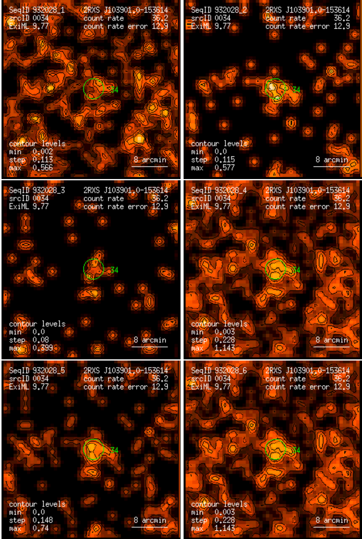
Figure 34: RASS 932028: detection 0034: band rate images, Gaussian filter: (1) PSPC channels 11 – 41, (2) 52 – 90, (3) 91 – 201, (4) 11 – 235, (5) 52 – 201, (6) 11 – 201. Broad band rates in counts/ks. Band rate contour levels in counts/ks/arcmin 2 .
