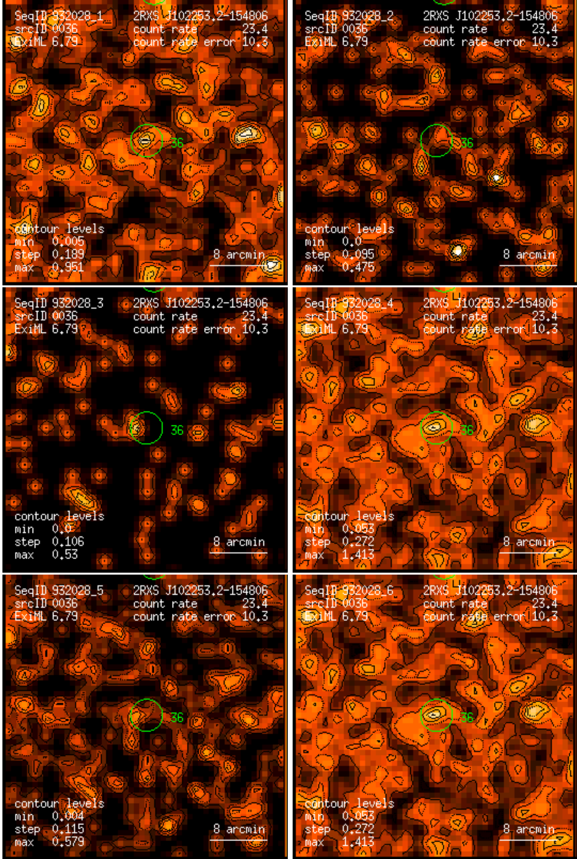
Figure 36: RASS 932028: detection 0036: band rate images, Gaussian filter: (1) PSPC channels 11 – 41, (2) 52 – 90, (3) 91 – 201, (4) 11 – 235, (5) 52 – 201, (6) 11 – 201. Broad band rates in counts/ks. Band rate contour levels in counts/ks/arcmin 2 .
