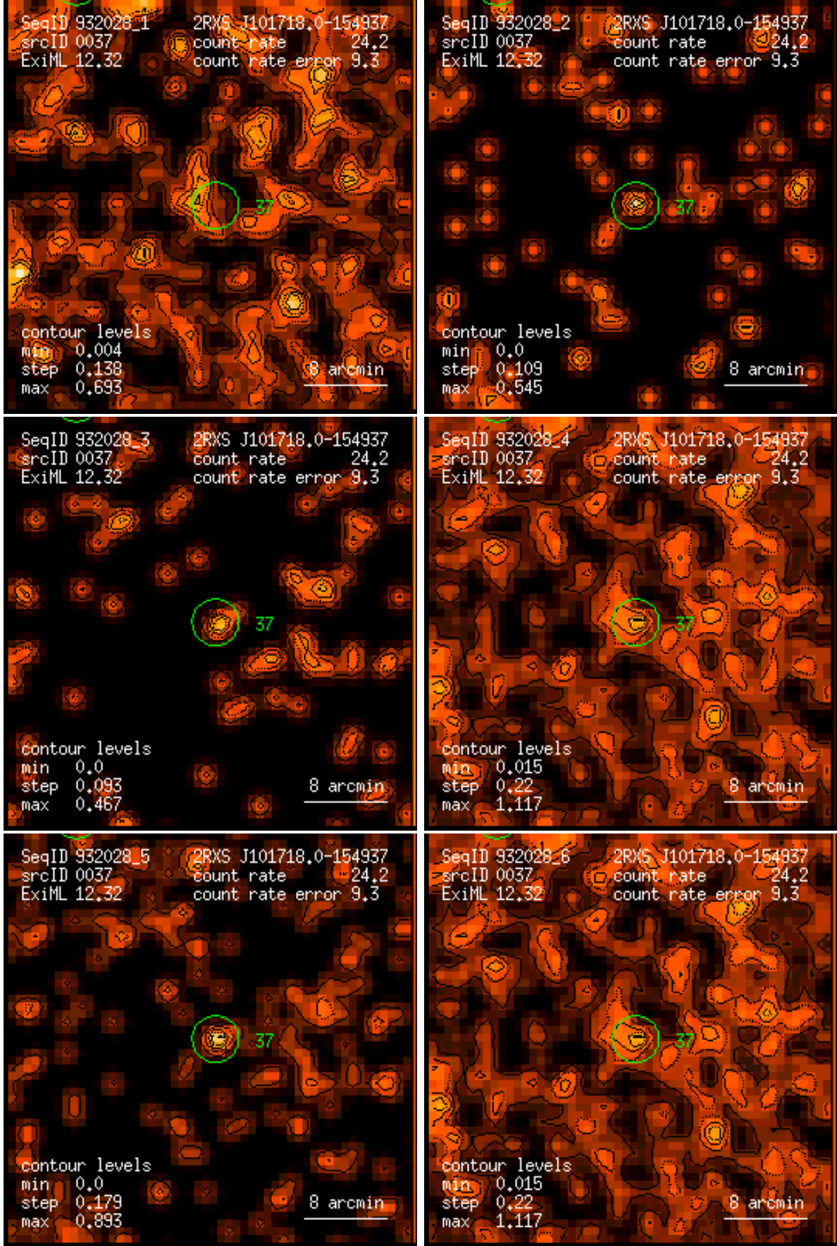
Figure 37: RASS 932028: detection 0037: band rate images, Gaussian filter: (1) PSPC channels 11 – 41, (2) 52 – 90, (3) 91 – 201, (4) 11 – 235, (5) 52 – 201, (6) 11 – 201. Broad band rates in counts/ks. Band rate contour levels in counts/ks/arcmin 2 .
