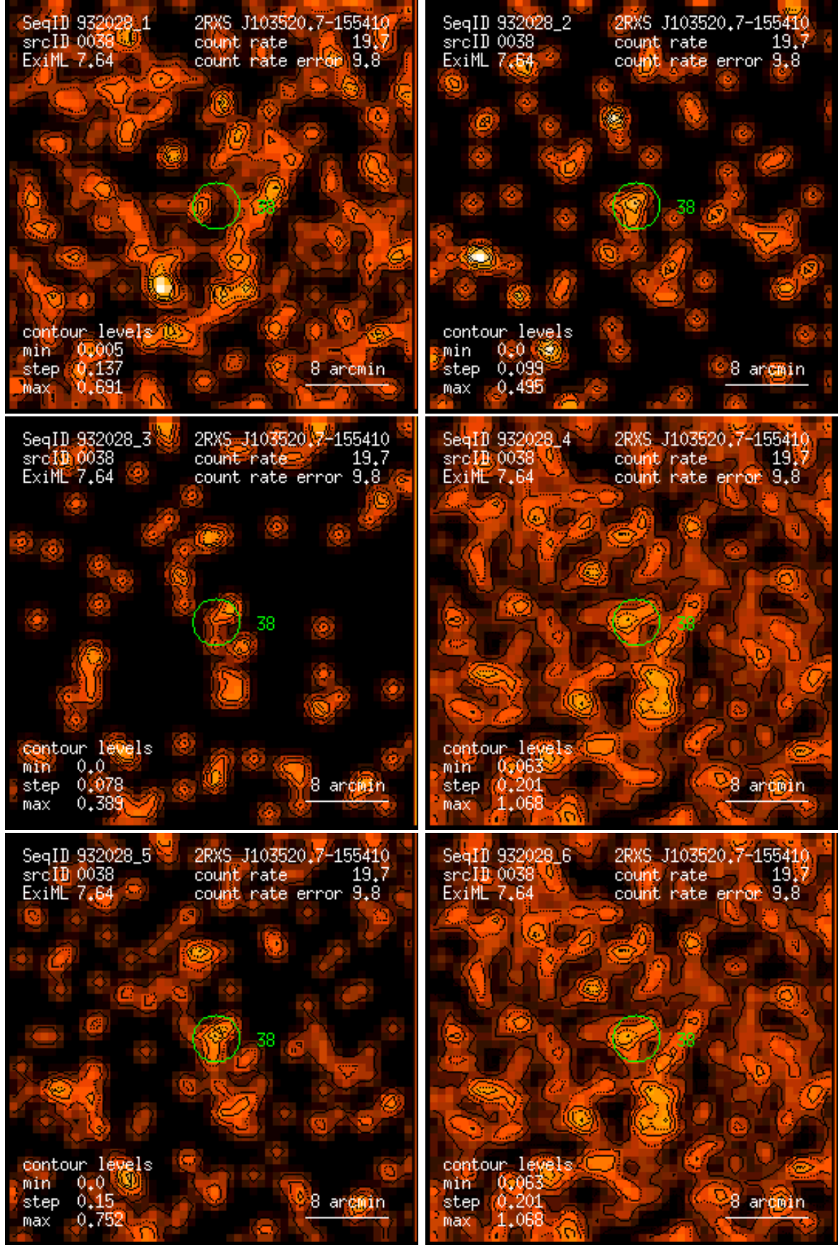
Figure 38: RASS 932028: detection 0038: band rate images, Gaussian filter: (1) PSPC channels 11 – 41, (2) 52 – 90, (3) 91 – 201, (4) 11 – 235, (5) 52 – 201, (6) 11 – 201. Broad band rates in counts/ks. Band rate contour levels in counts/ks/arcmin 2 .
