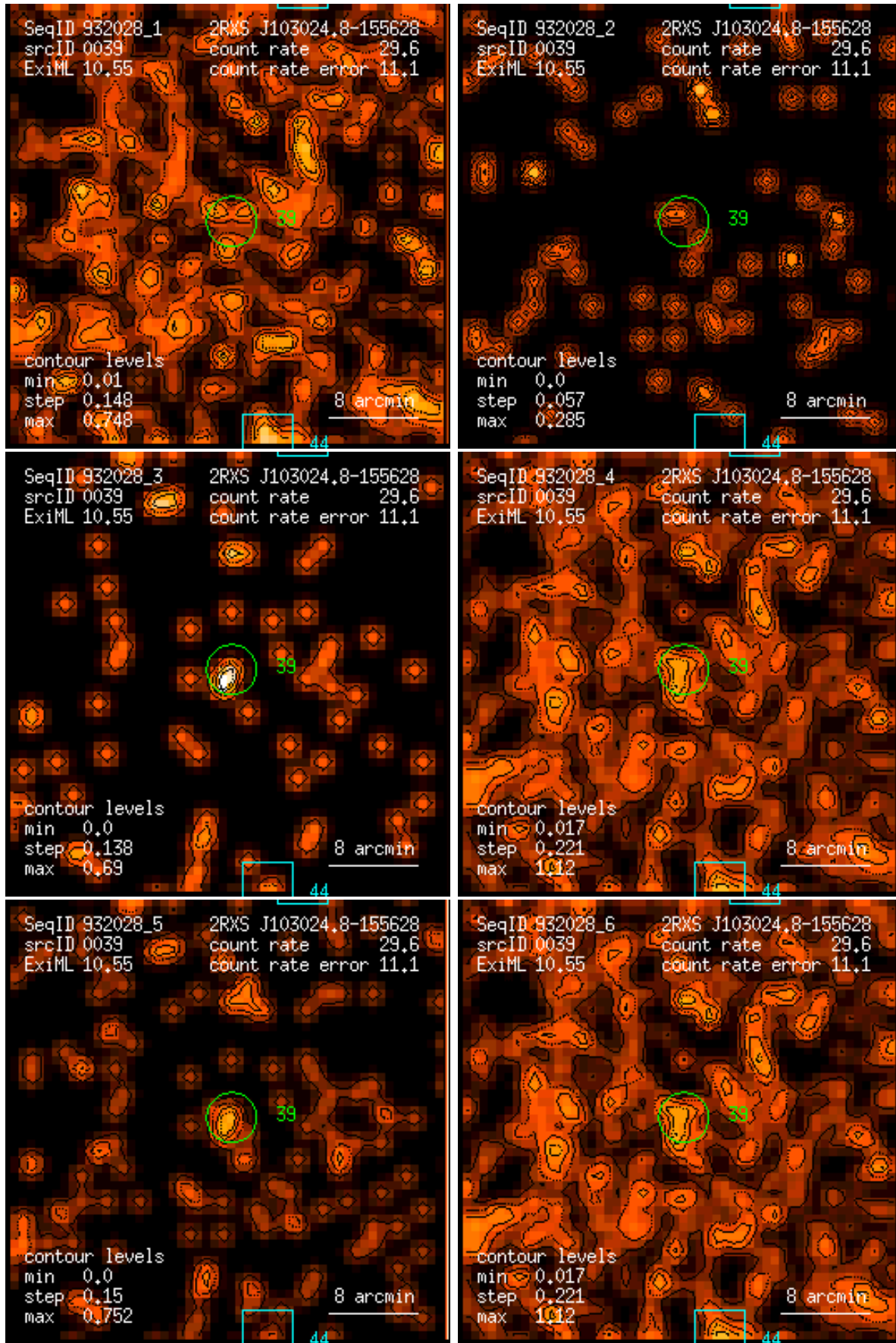
Figure 39: RASS 932028: detection 0039: band rate images, Gaussian filter: (1) PSPC channels 11 – 41, (2) 52 – 90, (3) 91 – 201, (4) 11 – 235, (5) 52 – 201, (6) 11 – 201. Broad band rates in counts/ks. Band rate contour levels in counts/ks/arcmin 2 .
