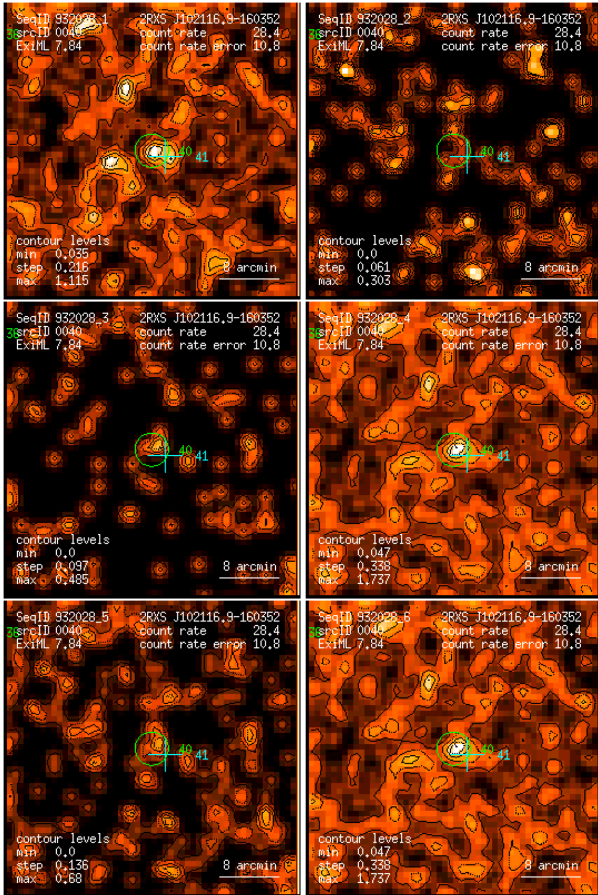
Figure 40: RASS 932028: detection 0040: band rate images, Gaussian filter: (1) PSPC channels 11 – 41, (2) 52 – 90, (3) 91 – 201, (4) 11 – 235, (5) 52 – 201, (6) 11 – 201. Broad band rates in counts/ks. Band rate contour levels in counts/ks/arcmin 2 .
