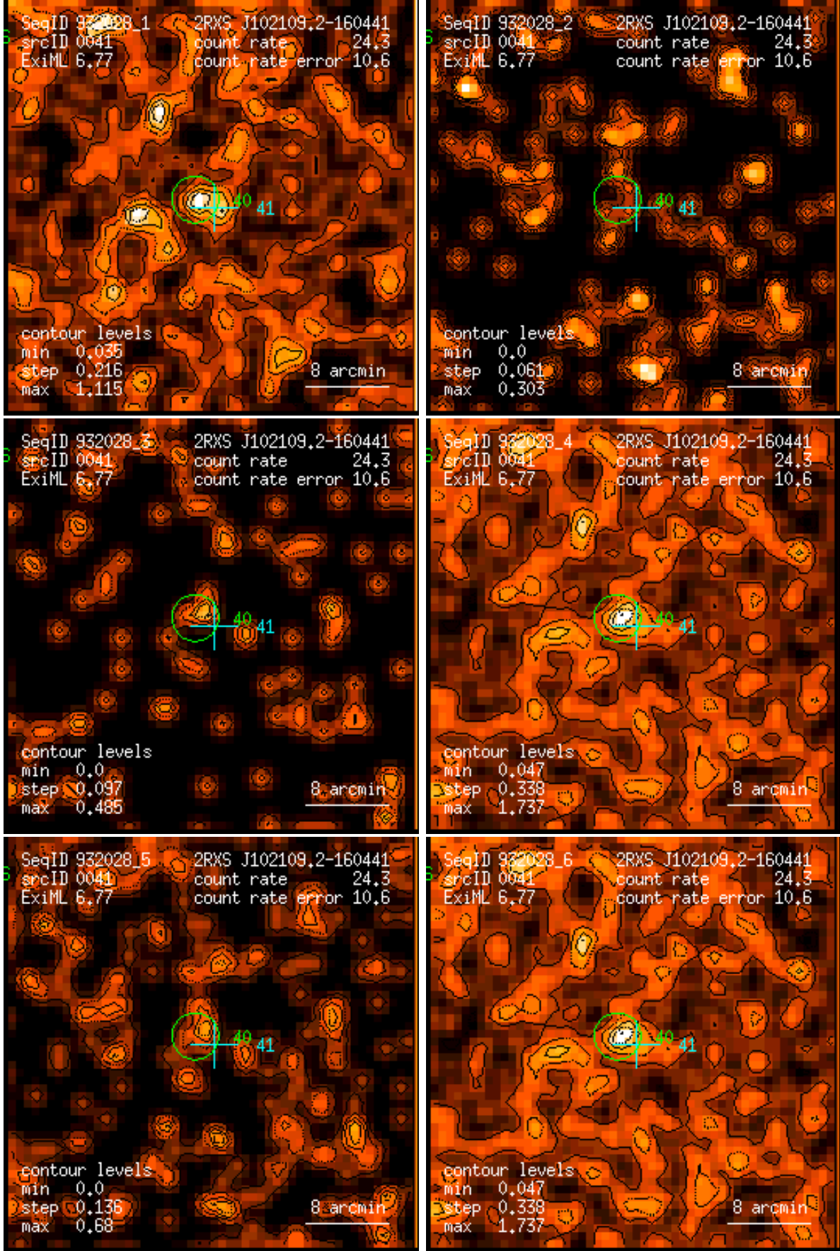
Figure 41: RASS 932028: detection 0041: band rate images, Gaussian filter: (1) PSPC channels 11 – 41, (2) 52 – 90, (3) 91 – 201, (4) 11 – 235, (5) 52 – 201, (6) 11 – 201. Broad band rates in counts/ks. Band rate contour levels in counts/ks/arcmin 2 .
