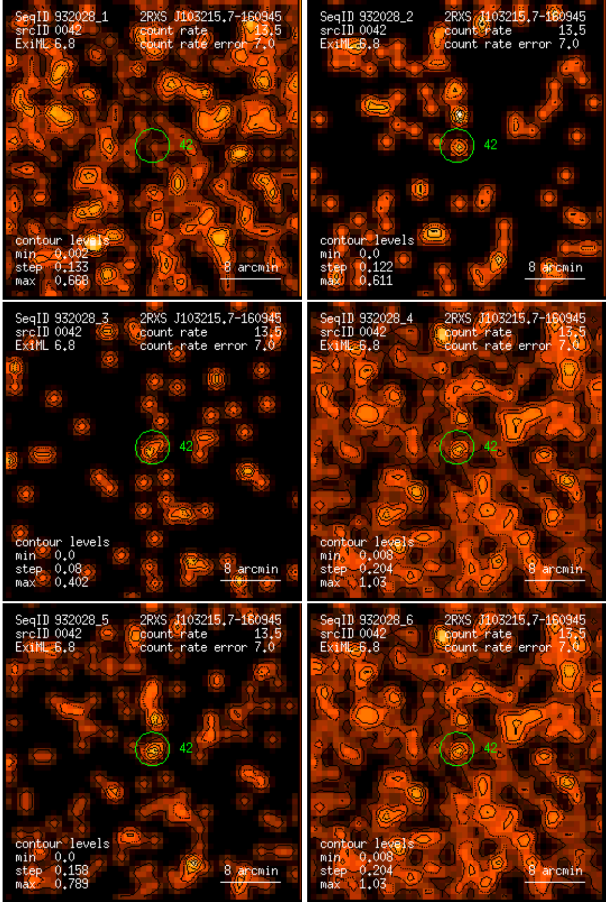
Figure 42: RASS 932028: detection 0042: band rate images, Gaussian filter: (1) PSPC channels 11 – 41, (2) 52 – 90, (3) 91 – 201, (4) 11 – 235, (5) 52 – 201, (6) 11 – 201. Broad band rates in counts/ks. Band rate contour levels in counts/ks/arcmin 2 .
