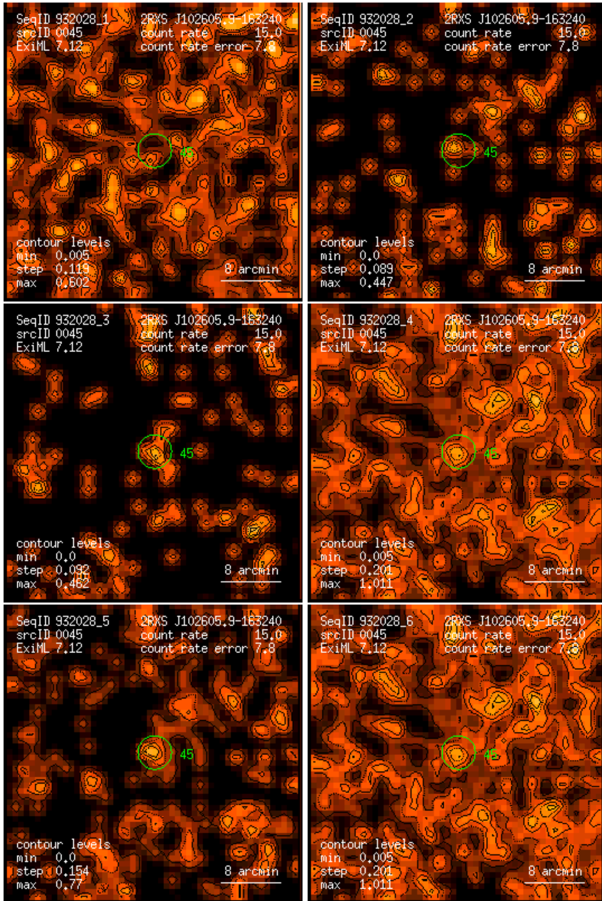
Figure 45: RASS 932028: detection 0045: band rate images, Gaussian filter: (1) PSPC channels 11 – 41, (2) 52 – 90, (3) 91 – 201, (4) 11 – 235, (5) 52 – 201, (6) 11 – 201. Broad band rates in counts/ks. Band rate contour levels in counts/ks/arcmin 2 .
