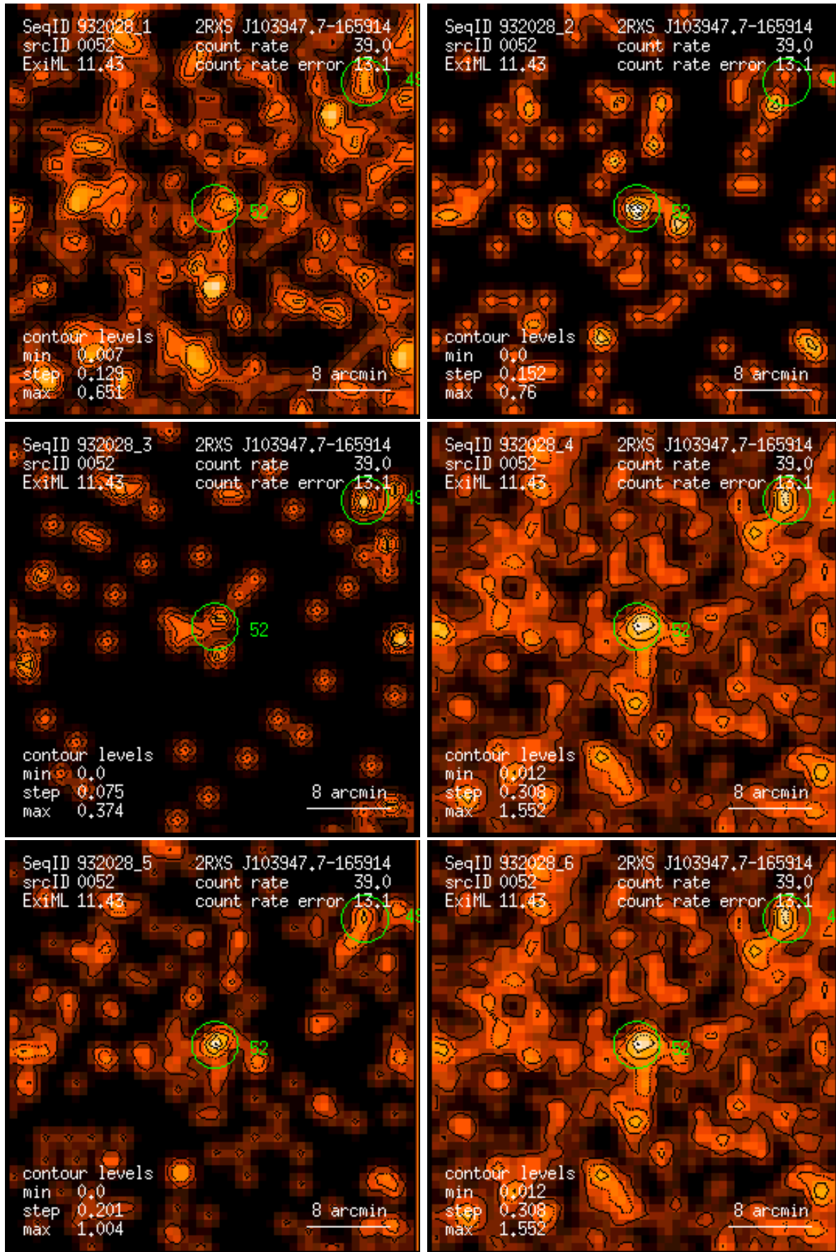
Figure 52: RASS 932028: detection 0052: band rate images, Gaussian filter: (1) PSPC channels 11 – 41, (2) 52 – 90, (3) 91 – 201, (4) 11 – 235, (5) 52 – 201, (6) 11 – 201. Broad band rates in counts/ks. Band rate contour levels in counts/ks/arcmin 2 .
