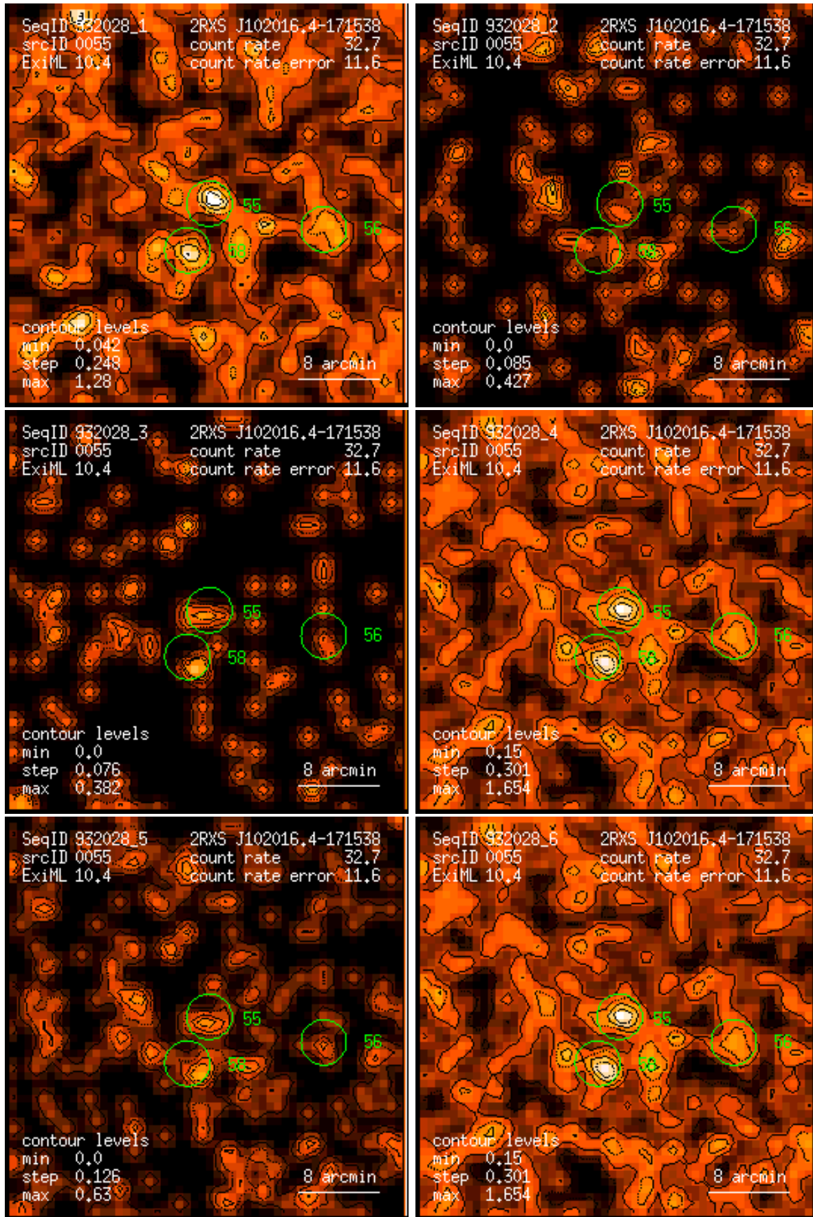
Figure 55: RASS 932028: detection 0055: band rate images, Gaussian filter: (1) PSPC channels 11 – 41, (2) 52 – 90, (3) 91 – 201, (4) 11 – 235, (5) 52 – 201, (6) 11 – 201. Broad band rates in counts/ks. Band rate contour levels in counts/ks/arcmin 2 .
