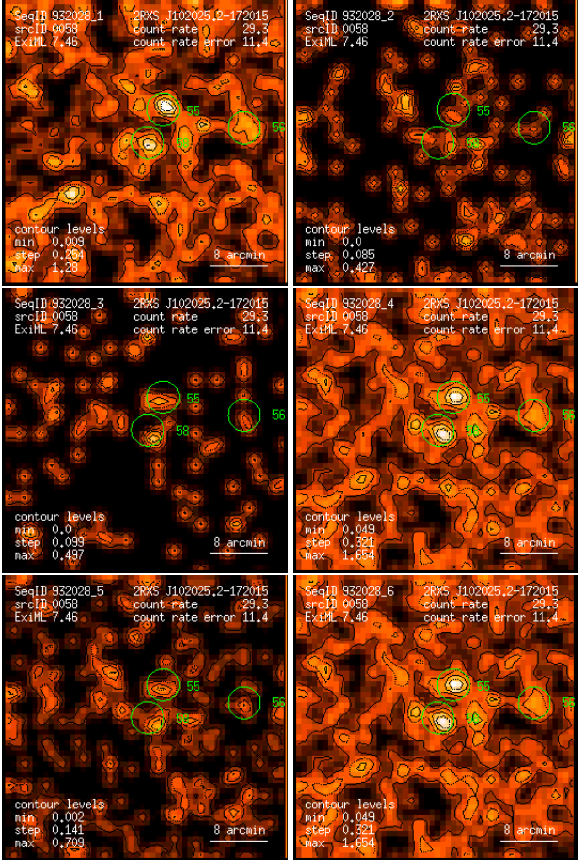
Figure 58: RASS 932028: detection 0058: band rate images, Gaussian filter: (1) PSPC channels 11 – 41, (2) 52 – 90, (3) 91 – 201, (4) 11 – 235, (5) 52 – 201, (6) 11 – 201. Broad band rates in counts/ks. Band rate contour levels in counts/ks/arcmin 2 .
