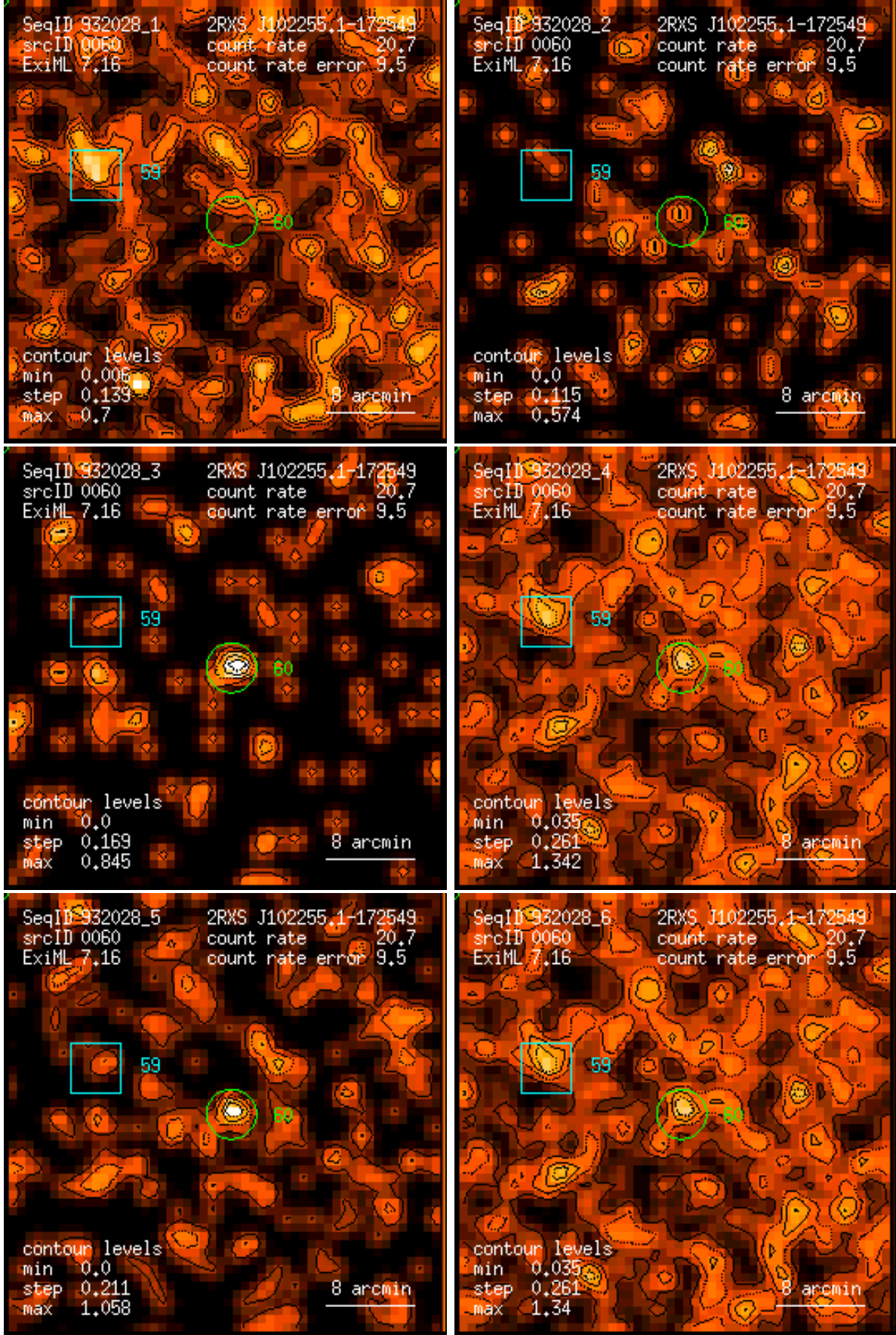
Figure 60: RASS 932028: detection 0060: band rate images, Gaussian filter: (1) PSPC channels 11 – 41, (2) 52 – 90, (3) 91 – 201, (4) 11 – 235, (5) 52 – 201, (6) 11 – 201. Broad band rates in counts/ks. Band rate contour levels in counts/ks/arcmin 2 .
