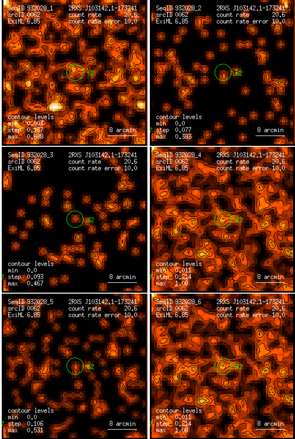
Figure 62: RASS 932028: detection 0062: band rate images, Gaussian filter: (1) PSPC channels 11 – 41, (2) 52 – 90, (3) 91 – 201, (4) 11 – 235, (5) 52 – 201, (6) 11 – 201. Broad band rates in counts/ks. Band rate contour levels in counts/ks/arcmin 2 .
