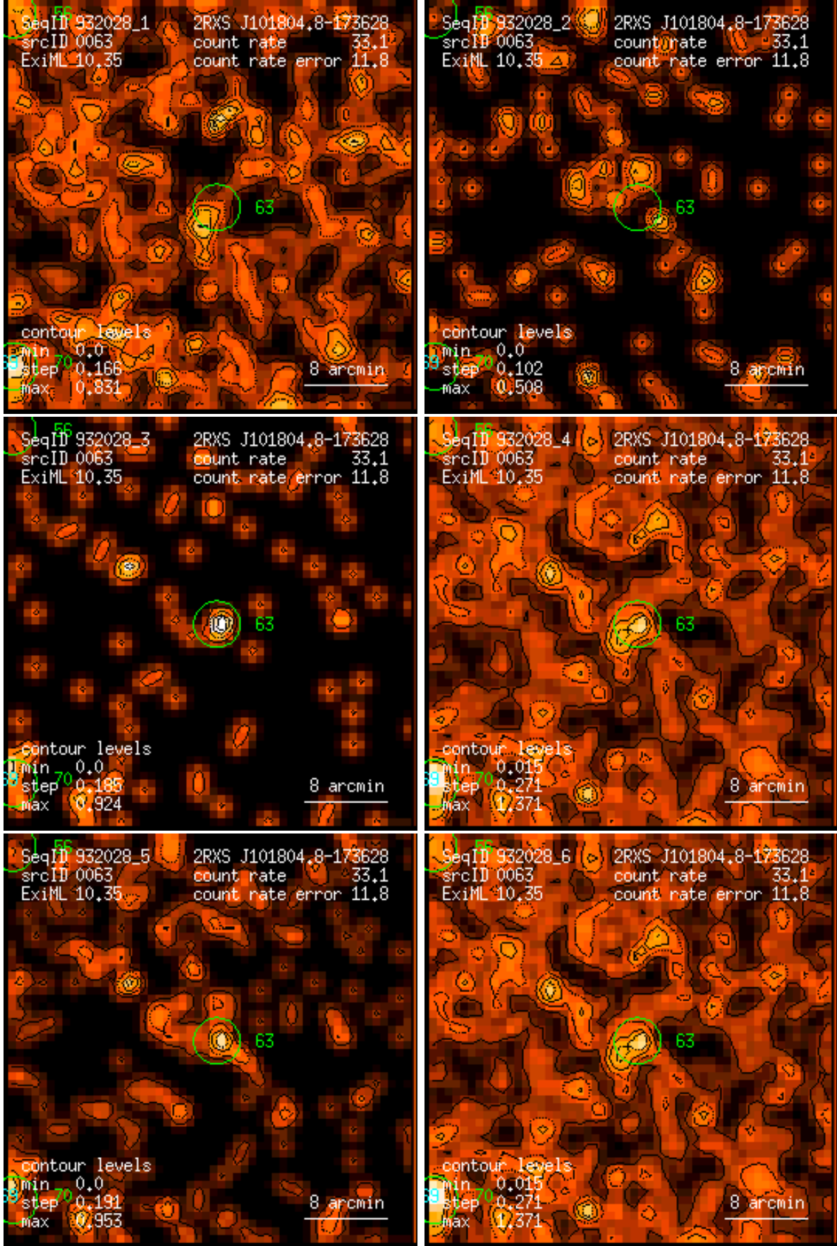
Figure 63: RASS 932028: detection 0063: band rate images, Gaussian filter: (1) PSPC channels 11 – 41, (2) 52 – 90, (3) 91 – 201, (4) 11 – 235, (5) 52 – 201, (6) 11 – 201. Broad band rates in counts/ks. Band rate contour levels in counts/ks/arcmin 2 .
