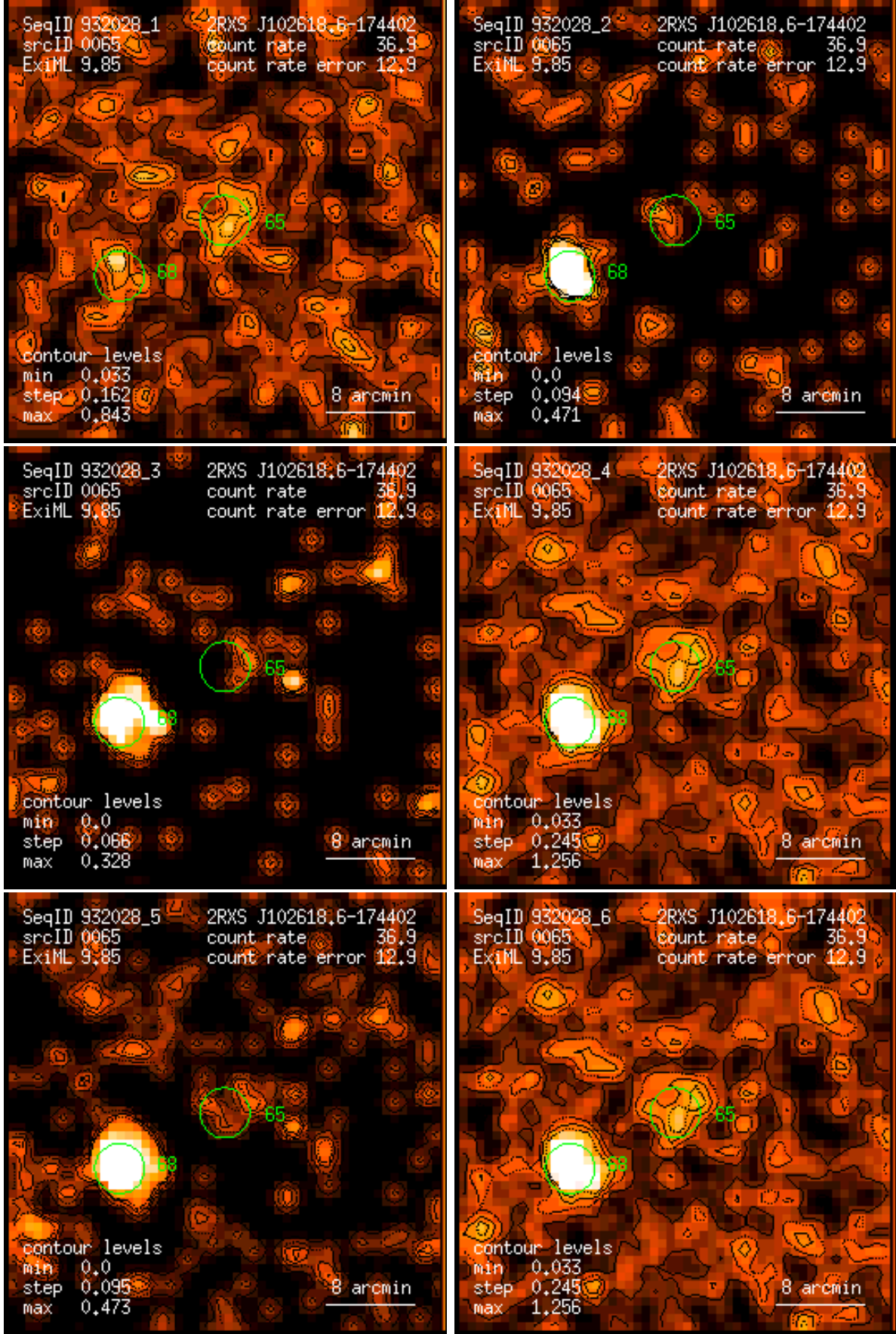
Figure 65: RASS 932028: detection 0065: band rate images, Gaussian filter: (1) PSPC channels 11 – 41, (2) 52 – 90, (3) 91 – 201, (4) 11 – 235, (5) 52 – 201, (6) 11 – 201. Broad band rates in counts/ks. Band rate contour levels in counts/ks/arcmin 2 .
