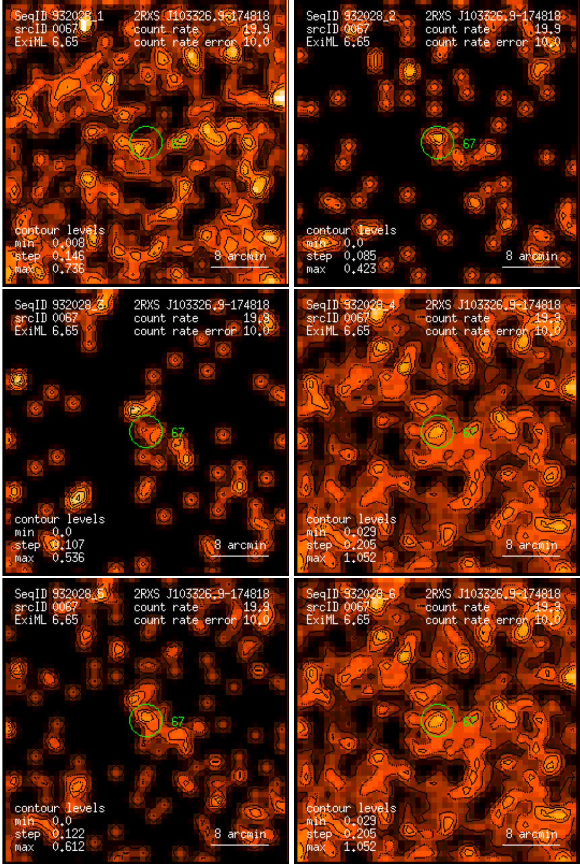
Figure 67: RASS 932028: detection 0067: band rate images, Gaussian filter: (1) PSPC channels 11 – 41, (2) 52 – 90, (3) 91 – 201, (4) 11 – 235, (5) 52 – 201, (6) 11 – 201. Broad band rates in counts/ks. Band rate contour levels in counts/ks/arcmin 2 .
