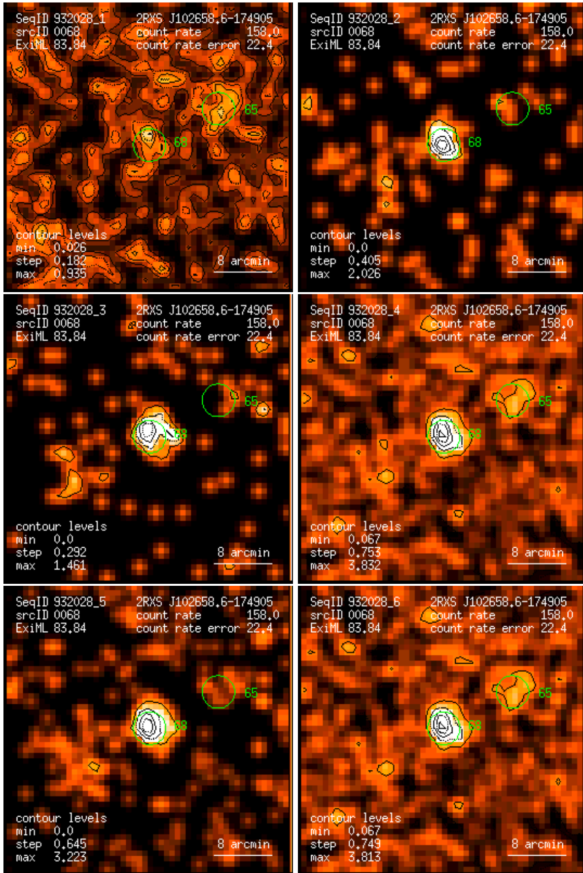
Figure 68: RASS 932028: detection 0068: band rate images, Gaussian filter: (1) PSPC channels 11 – 41, (2) 52 – 90, (3) 91 – 201, (4) 11 – 235, (5) 52 – 201, (6) 11 – 201. Broad band rates in counts/ks. Band rate contour levels in counts/ks/arcmin 2 .
