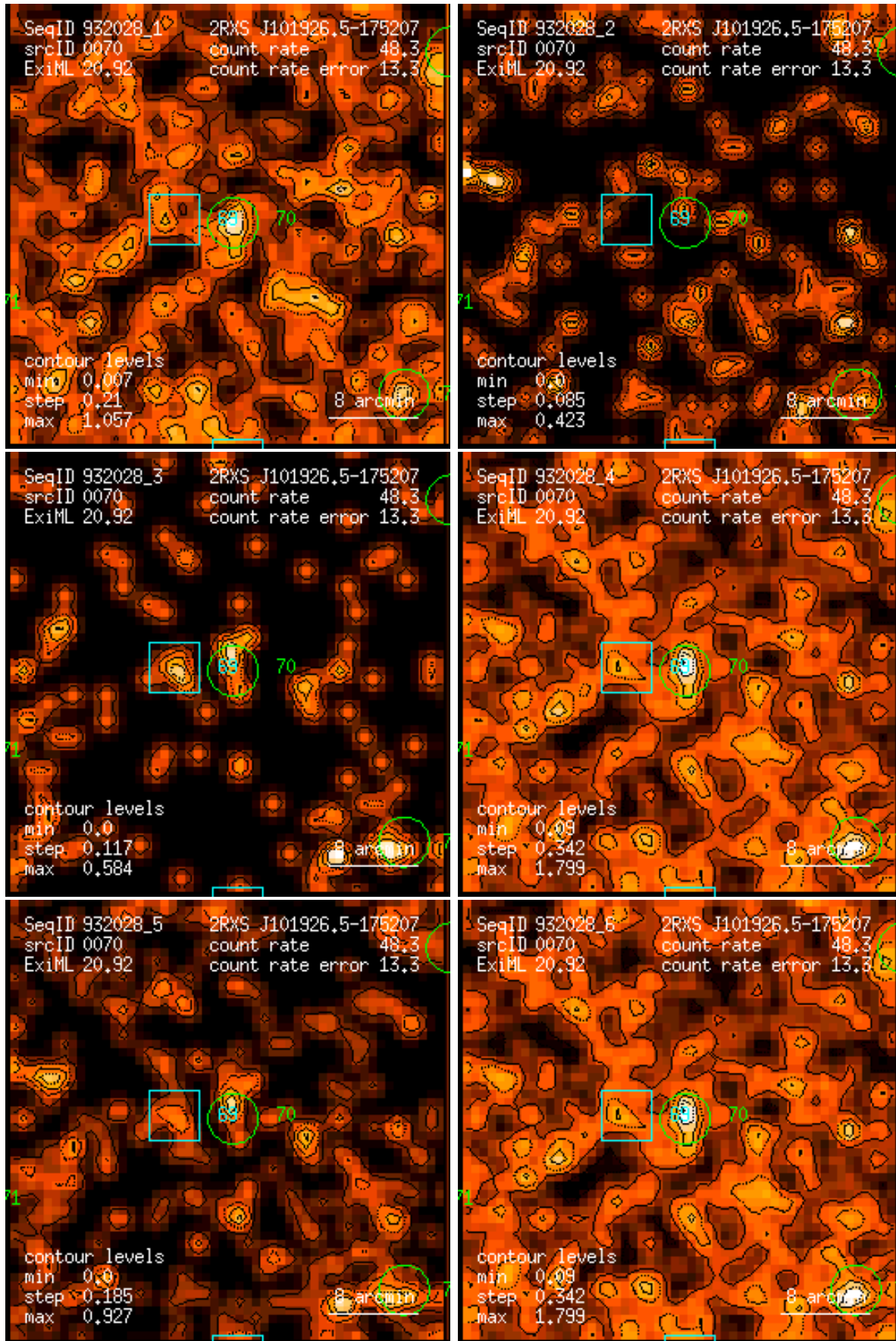
Figure 70: RASS 932028: detection 0070: band rate images, Gaussian filter: (1) PSPC channels 11 – 41, (2) 52 – 90, (3) 91 – 201, (4) 11 – 235, (5) 52 – 201, (6) 11 – 201. Broad band rates in counts/ks. Band rate contour levels in counts/ks/arcmin 2 .
