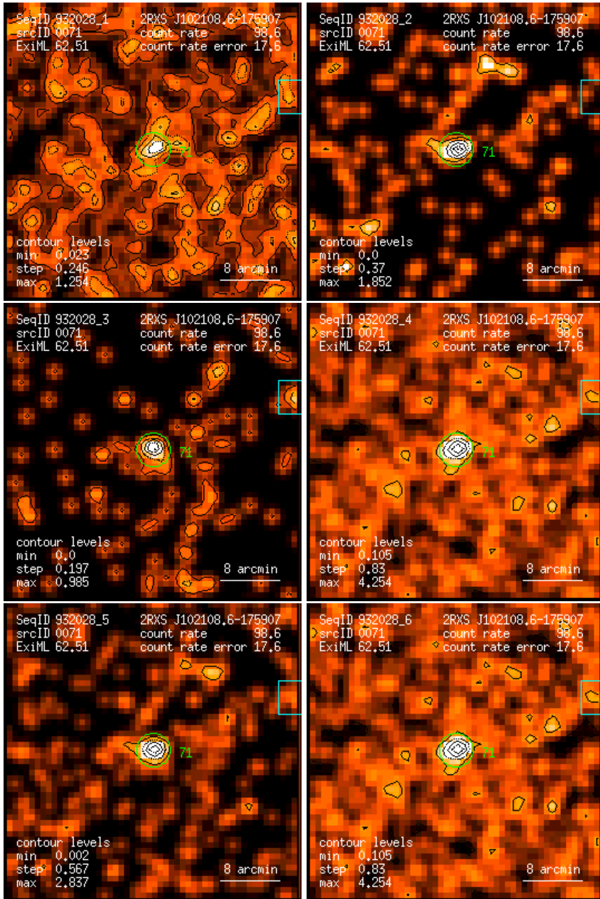
Figure 71: RASS 932028: detection 0071: band rate images, Gaussian filter: (1) PSPC channels 11 – 41, (2) 52 – 90, (3) 91 – 201, (4) 11 – 235, (5) 52 – 201, (6) 11 – 201. Broad band rates in counts/ks. Band rate contour levels in counts/ks/arcmin 2 .
