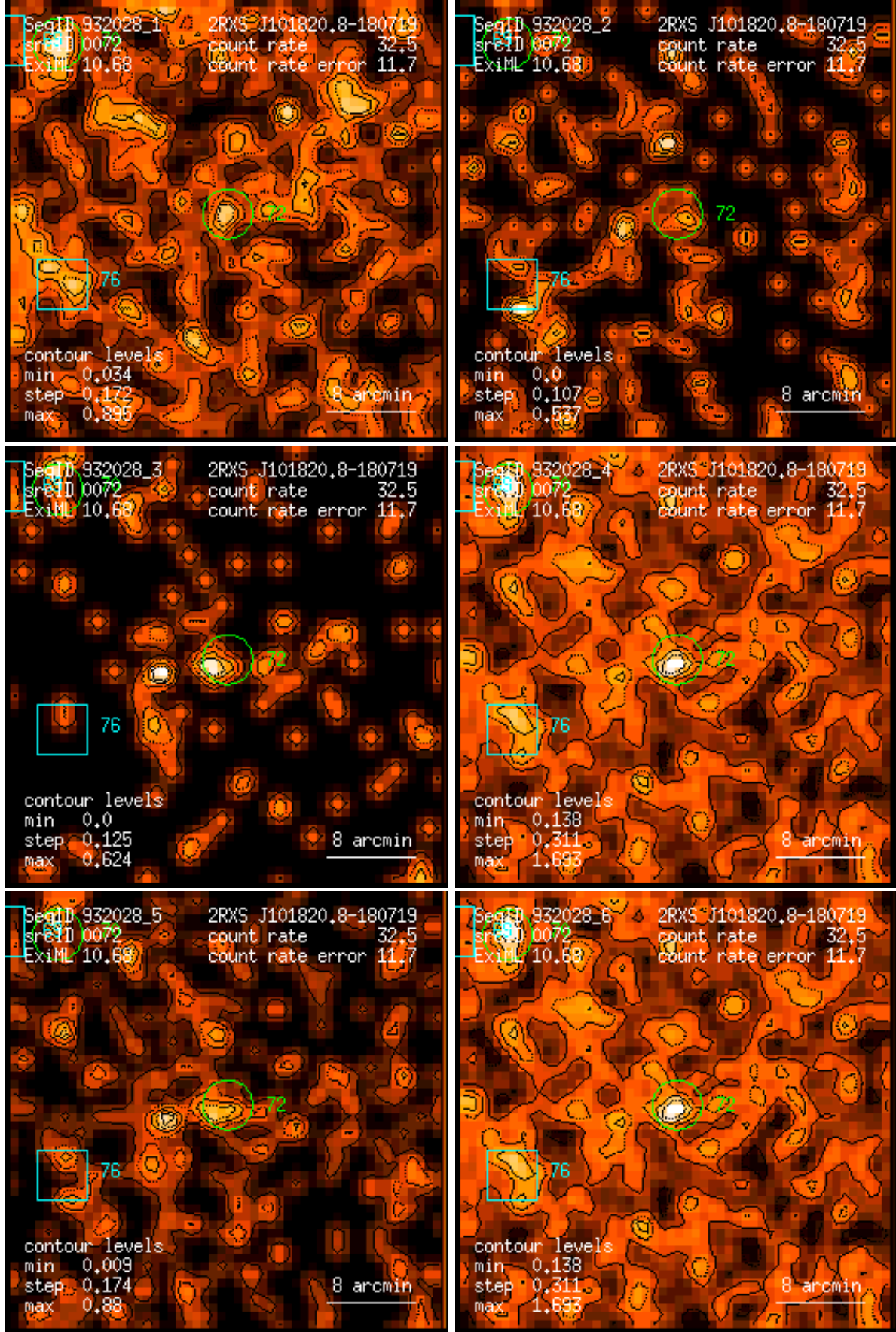
Figure 72: RASS 932028: detection 0072: band rate images, Gaussian filter: (1) PSPC channels 11 – 41, (2) 52 – 90, (3) 91 – 201, (4) 11 – 235, (5) 52 – 201, (6) 11 – 201. Broad band rates in counts/ks. Band rate contour levels in counts/ks/arcmin 2 .
