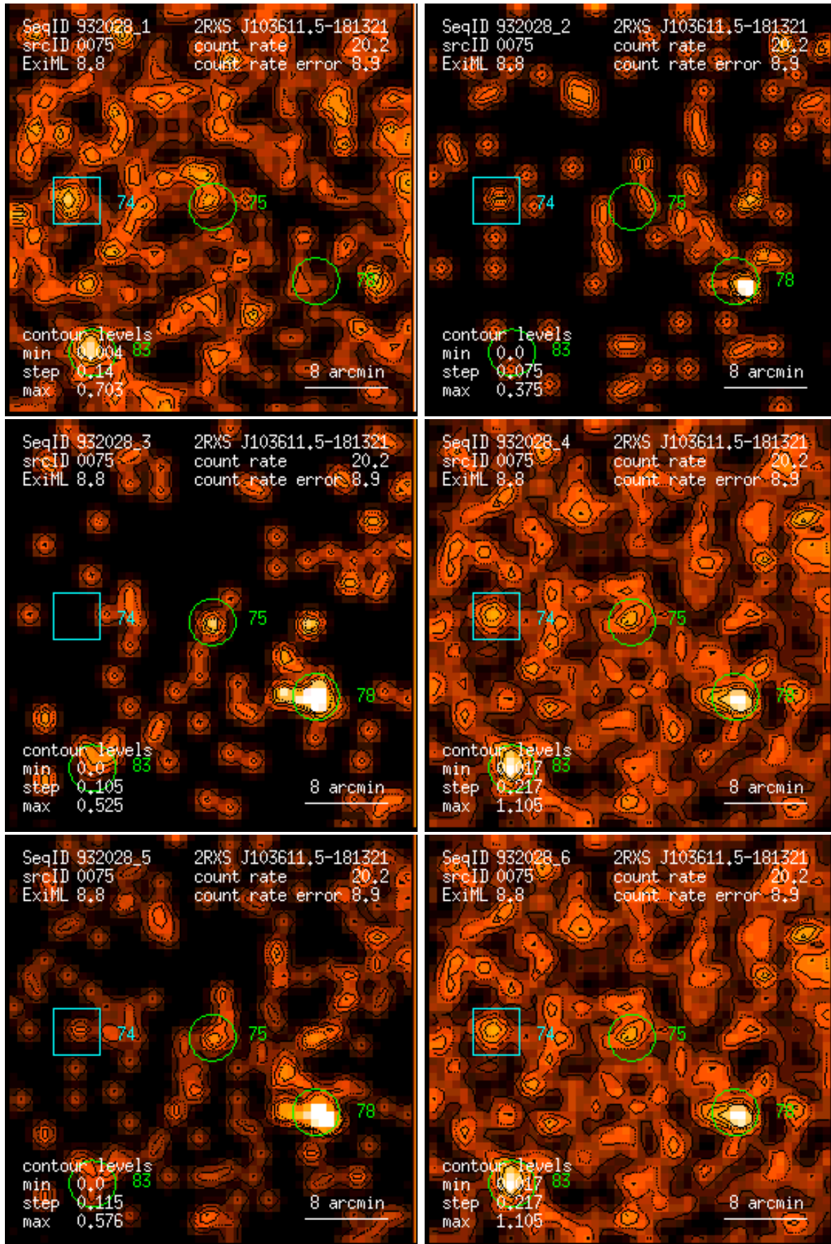
Figure 75: RASS 932028: detection 0075: band rate images, Gaussian filter: (1) PSPC channels 11 – 41, (2) 52 – 90, (3) 91 – 201, (4) 11 – 235, (5) 52 – 201, (6) 11 – 201. Broad band rates in counts/ks. Band rate contour levels in counts/ks/arcmin 2 .
