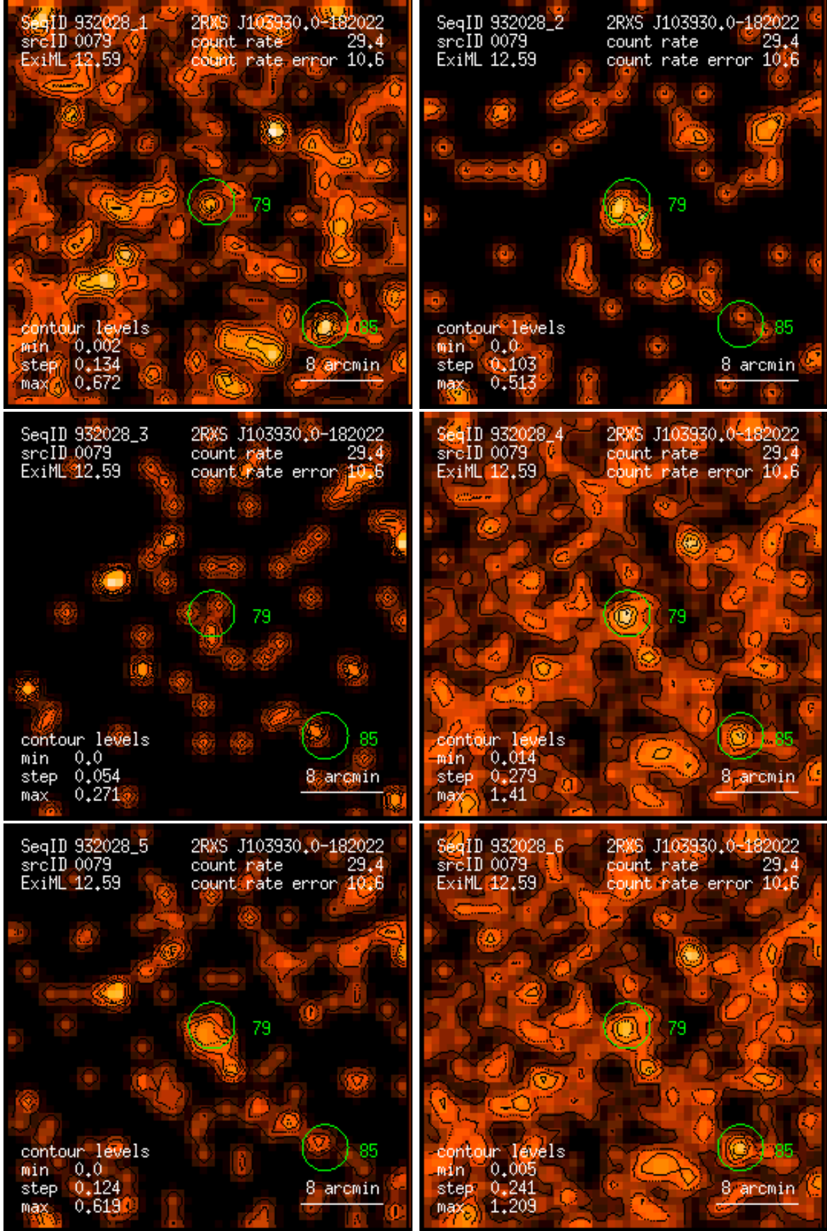
Figure 79: RASS 932028: detection 0079: band rate images, Gaussian filter: (1) PSPC channels 11 – 41, (2) 52 – 90, (3) 91 – 201, (4) 11 – 235, (5) 52 – 201, (6) 11 – 201. Broad band rates in counts/ks. Band rate contour levels in counts/ks/arcmin 2 .
