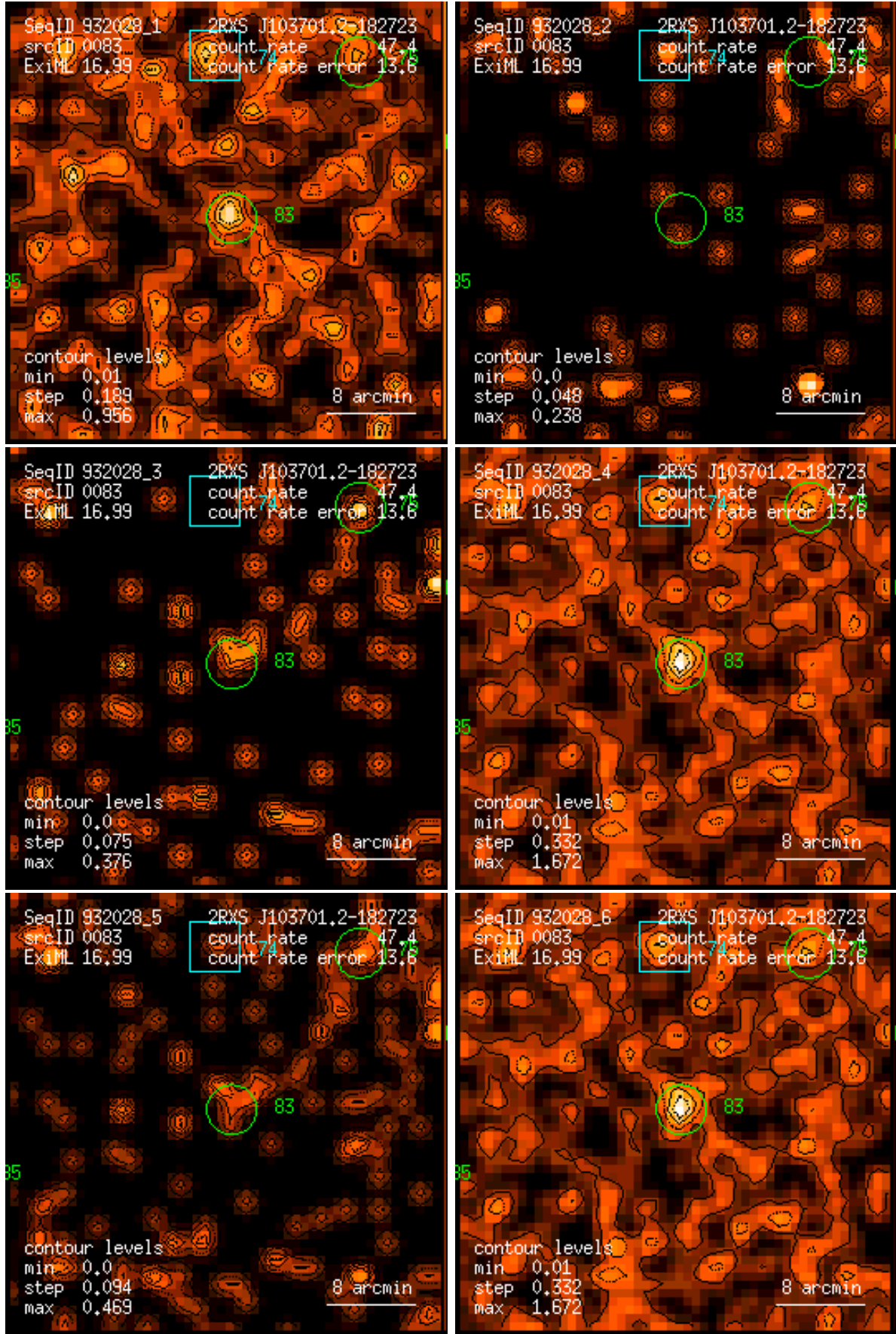
Figure 83: RASS 932028: detection 0083: band rate images, Gaussian filter: (1) PSPC channels 11 – 41, (2) 52 – 90, (3) 91 – 201, (4) 11 – 235, (5) 52 – 201, (6) 11 – 201. Broad band rates in counts/ks. Band rate contour levels in counts/ks/arcmin 2 .
